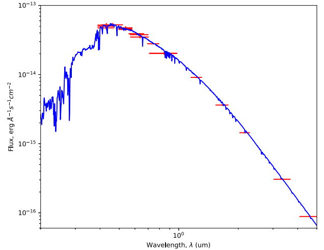
Figure 11. The APASS ( B , V , g' , r' , i' ), 2MASS ( J , H , K_s ), WISE (W1, W2), MASTER ( B , V , R , I ), and TRAPPIST-North ( B , V , R_c , I_c ) spectral points are shown. The blue curve is a model for the star with T_{\text{eff}} = 7200 \text{ K} , R_* = 1.64 R_\odot , \log g_* = 4.2 and [\text{Fe}/\text{H}] = 0.43 at 655 pc and E(B - V) = 0.18 .
