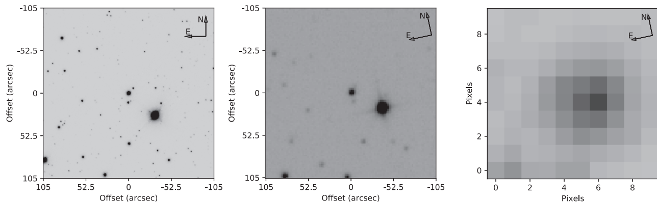
Figure 1. Left: Pan-STARRS i' image of a 210 \times 210 \text{ arcsec}^2 region around GPX-1 ( V \sim 12 mag), obtained with an image scale of 0.25 \text{ arcsec pixel}^{-1} . Note the bright star HD 15691 ( V \sim 9 mag) located 42 arcsec SW from GPX-1. Middle: image of the same field obtained with a telescope with an image scale of 1.85 \text{ arcsec pixel}^{-1} . Right: TESS 210 \times 210 \text{ arcsec}^2 ( 10 \times 10 \text{ pixel}^2 ) image of the same field of view (FoV).
