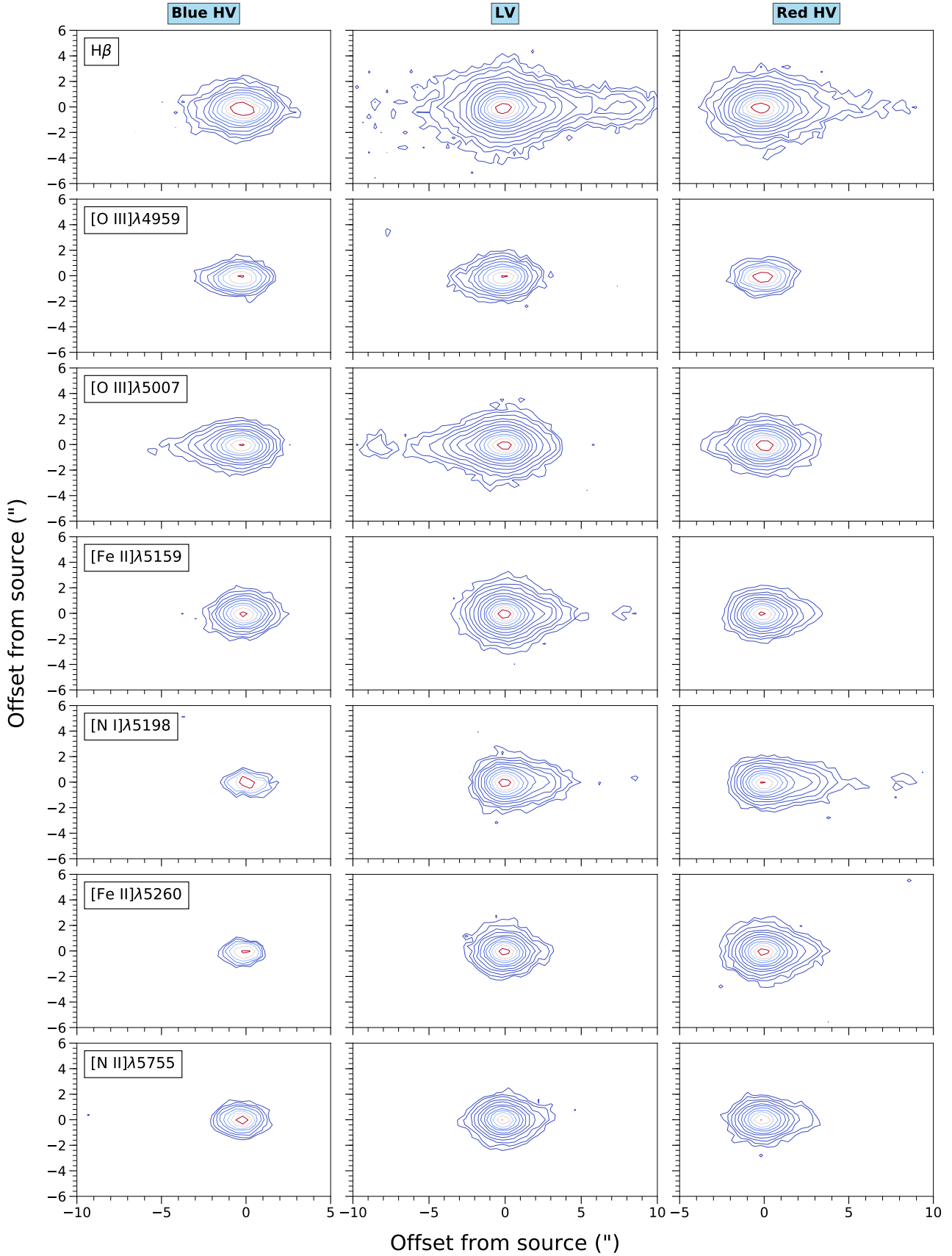
Fig. A.2. Spectroimages showing selected emission lines shown in three channels: the blue-shifted HV ( -150 to -90 \text{km s}^{-1} ); centre, the low-velocity channel ( \pm 90 \text{km s}^{-1} ); and the red-shifted HV ( +90 to -150 \text{km s}^{-1} ). Contours begin at 3\text{-}\sigma of the background noise and increase as factors of \sqrt{3} .
