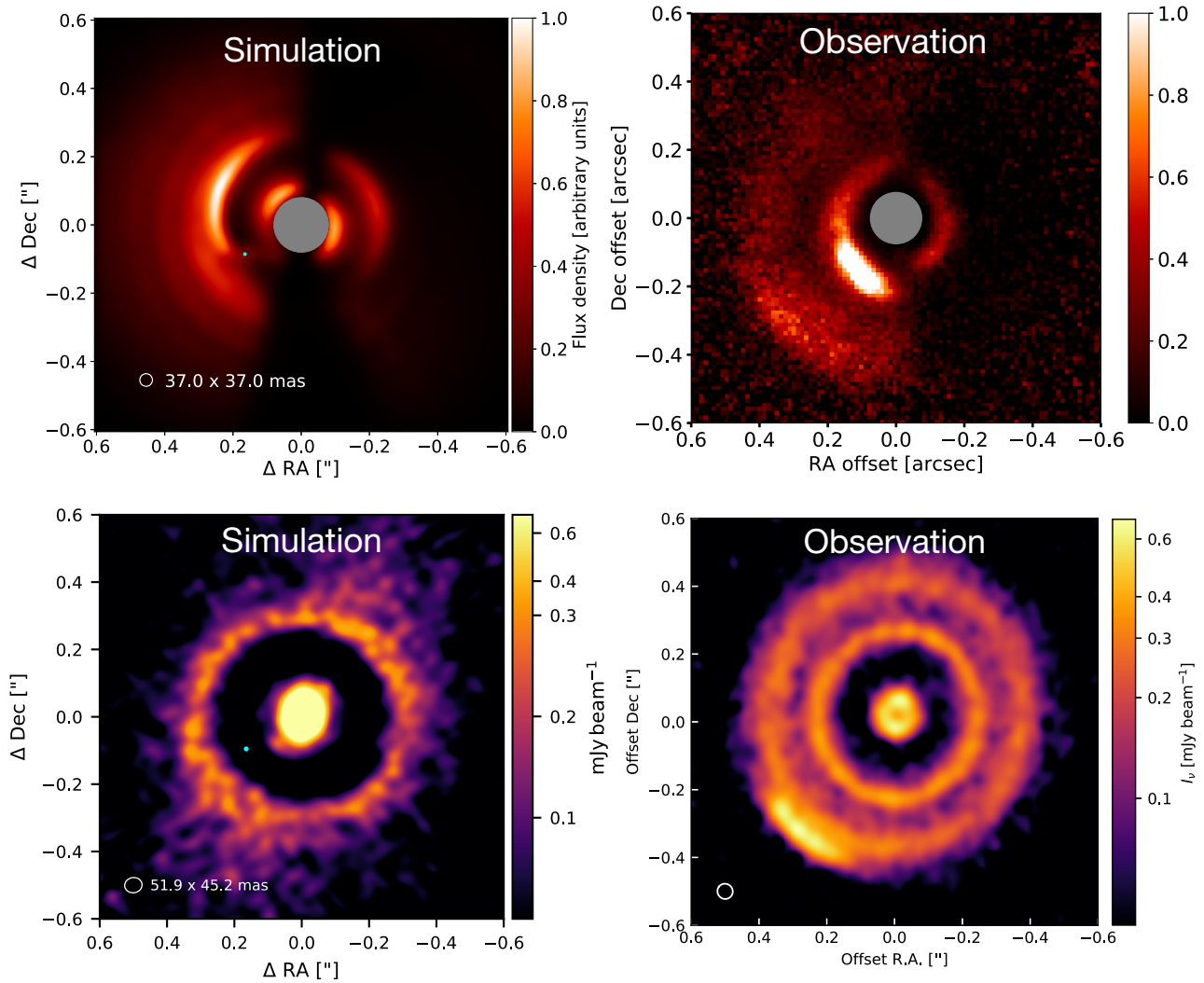
Figure 5. Comparison between the results from our ‘binary + planet’ model (left-hand panels) and the observations (right-hand panels). Top panels: Polarized intensity image Q_{\Phi} observed at 1.2 \mu\text{m} ( J band) of the hydro simulation of HD 143006. The flux has been scaled by r^2 to enhance the drop in intensity. The grey circle indicates the 0.08 arcsec coronagraphic mask. The image on the right has been taken from Benisty et al. (2018). 1 Bottom panels: ALMA Band 6 synthetic observation at 1.3 mm of the dust continuum emission. The empty circles in the bottom left corners indicate the corresponding beam size. The image on the right has been taken from Pérez et al. (2018). 2
