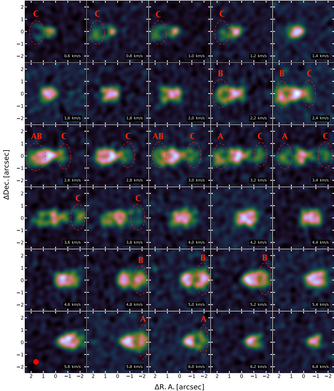
Fig. 3. Channel maps of the CN emission in the Flying Saucer from 0.60 to 6.40 \text{km s}^{-1} with the velocity labels referring to the B component. The spectral resolution is 0.2 \text{ km s}^{-1} and the rms per channel is 14 \text{ mJy beam}^{-1} . The synthesized beam size is represented in the lower left panel . The frequency range covers the A, B, and C HF components, which are J = 5/2 \rightarrow 3/2 and F = 5/2 \rightarrow 3/2 , J = 5/2 \rightarrow 3/2 and F = 7/2 \rightarrow 5/2 , and J = 5/2 \rightarrow 3/2 and F = 3/2 \rightarrow 1/2 , respectively, and are listed in Table 1.
