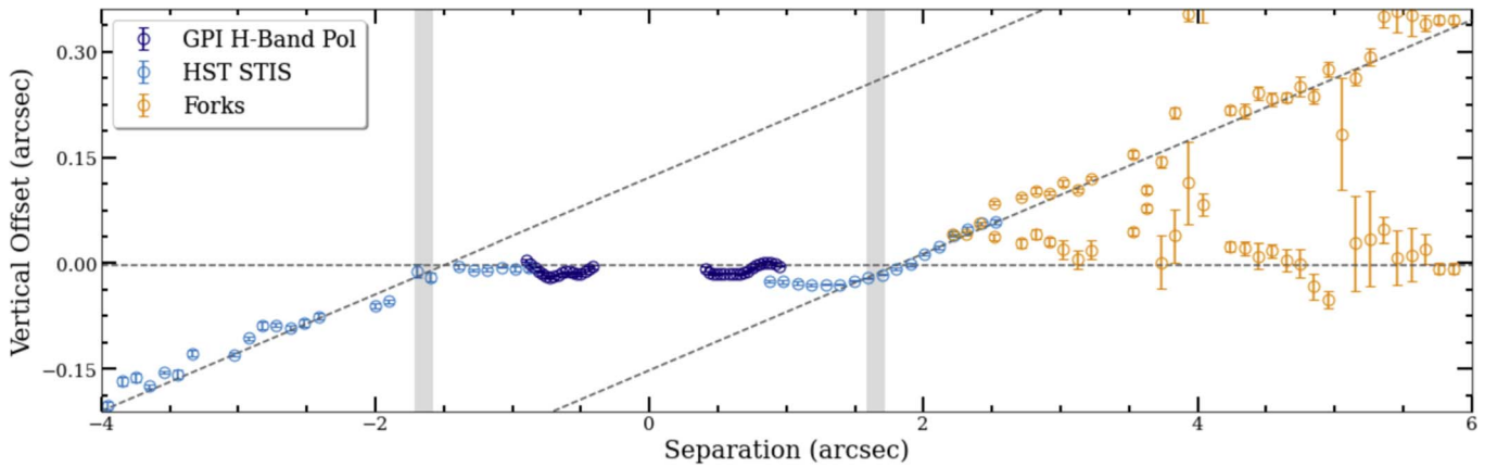
Figure 5. Vertical offset profiles of the GPI and HST data for HD 111520. Both images are rotated by 75^{\circ}.7 clockwise. The dark blue data points represents the GPI vertical offset in the pol H band, the light blue data points represents the HST vertical offset, while the orange data points represent the vertical offset of the bifurcation or fork feature observed with HST in the NW extension. The diagonal gray dashed lines are plotted to show the slopes of the SE and NW extensions of the disk halo seen with HST, while the horizontal gray dashed line shows the alignment of the GPI data. The vertical shaded regions at 1^{\prime}.7 show where the disk halo changes from being relatively flat to sloped.
