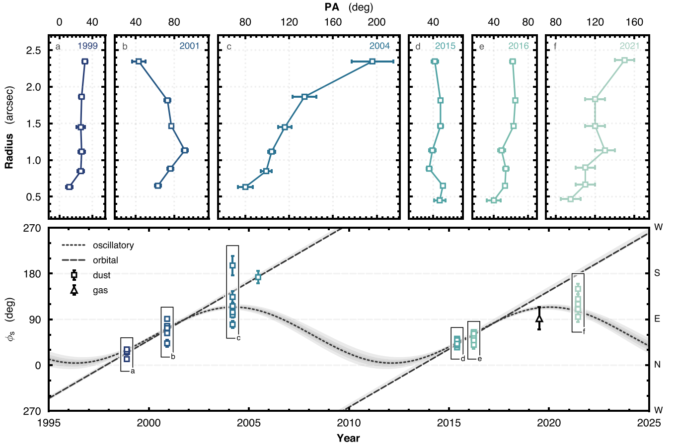
Figure 3. Summary of the temporal evolution of the shadow. The top row shows the six epochs where the shadow has been radially resolved in HST data (Debes et al. 2017), all sharing the same x-axis scaling. The bottom panel shows the azimuthal location of the shadow as a function of time. Two different models of the time evolution of the shadow are shown: a regular orbit, Equation (3), shown by the dashed line, or oscillatory motion, Equation (4), shown by the dotted line. The shaded regions about both lines show \pm 3\sigma about the median value of the posterior. Square points show epoch-median shadows observed in the scattered light, with each symbol representing a separate radial bin. The triangle symbol shows the median shadow location beyond 3'' observed in the gas with ALMA.
