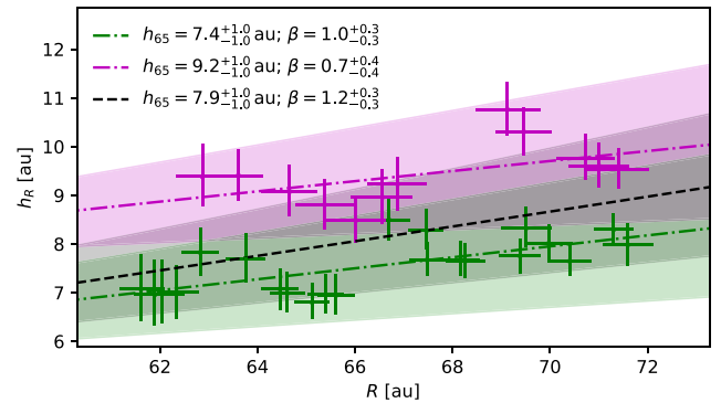
Figure 10. Apparent height of the scattering surface, h_{\text{scat}}(r) , as a function of the elliptical ring radius, r (data are from Table 1: magenta and green data points are from fits to the J -band and H -band isophotes, respectively). The dashed lines show the best-fitting power law profiles (equation 7) to the H -band (green line), the J -band (magenta line), and the combined J - and H -band data (black line). The amplitude, h_{65} , and exponent, \beta , of the power law fits are provided in the legend.
