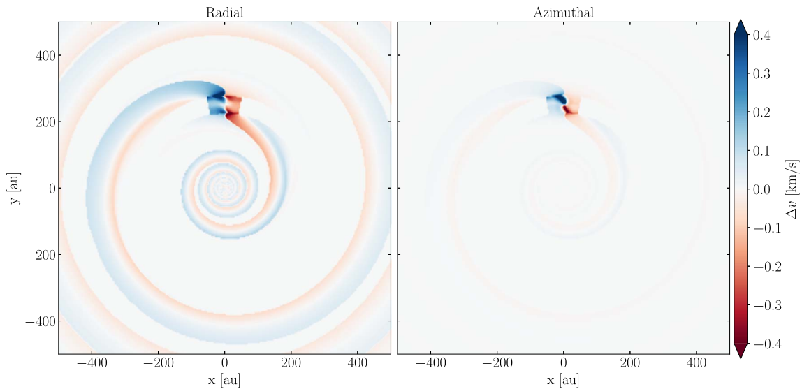
Figure 2. Analytic prediction of the velocity perturbation generated by the planetary wake of a 3 M_J planet located at 250 au. The left and right panels show radial and azimuthal velocity perturbations, respectively. Note that positive radial velocities indicate motion away from the central star, and positive azimuthal velocities indicate super-Keplerian flow.
