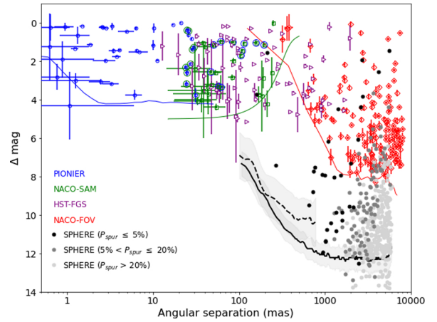
Fig. 12. \Delta\text{mag} vs. separation diagram. The location of the newly discovered sources (black and grey dots), as well as the median IRDIS and IFS contrast limits are compared with the outcome of previous surveys (Sana et al. 2014). Black, grey, and light-grey dots corresponds to sources with P_{\text{spur}} \leq 5\% , 5\% < P_{\text{spur}} \leq 20\% , and P_{\text{spur}} > 20\% , respectively.
