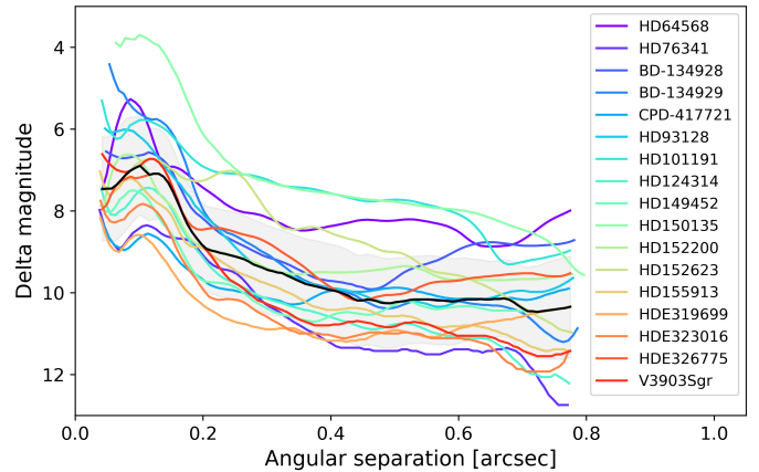
Fig. 10. Sensitivity of our IFS observations expressed as magnitude difference vs. angular separation to the central star. The curves for each objects correspond to the 5\text{-}\sigma contrast.
