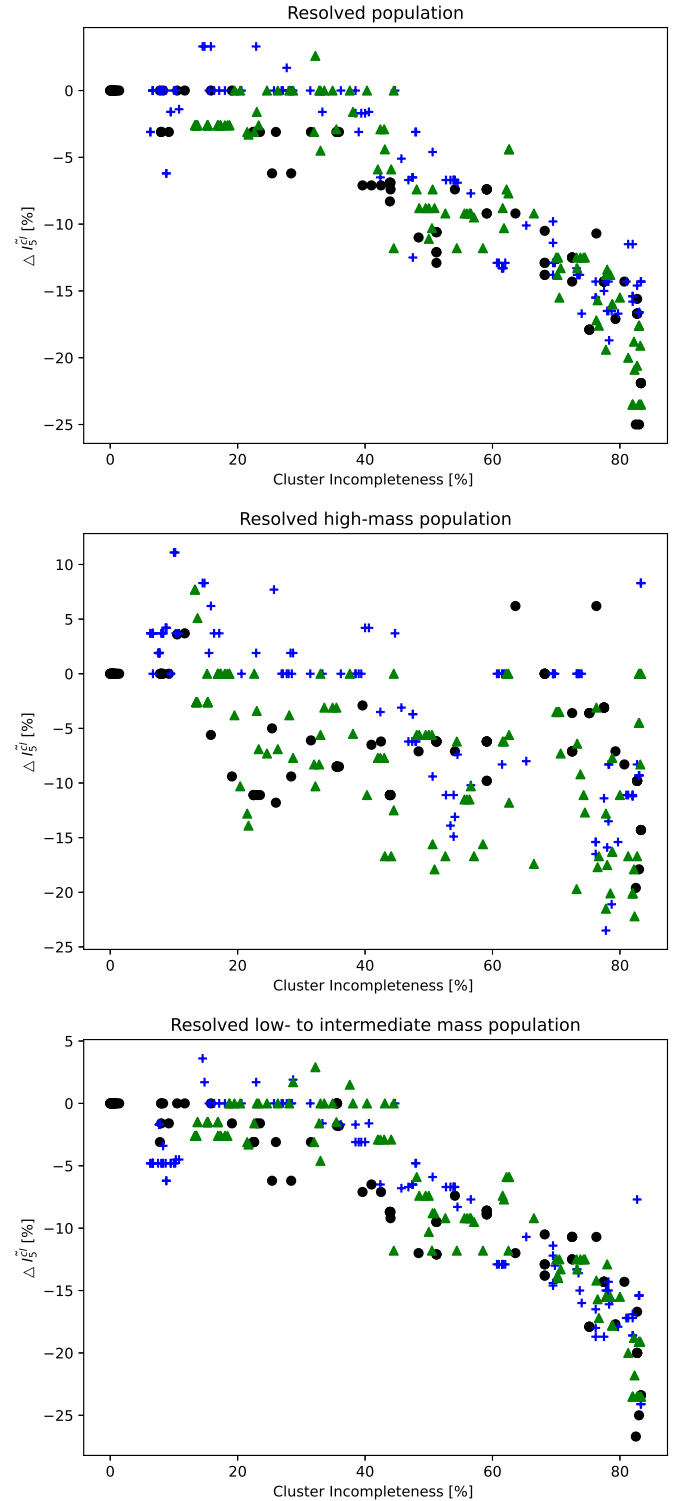
Fig. 4. Change in the median index value derived for stars identified as spatially clustered, \tilde{I}_5^{\text{cl}} , in the resolved populations: top panel : general, middle panel : high-mass, and bottom panel : low- to intermediate-mass. Symbols and colours indicate the binary fraction of the host cluster: f = 0.0 (black circles), f = 0.25 (blue crosses), f = 0.5 (green triangles).
