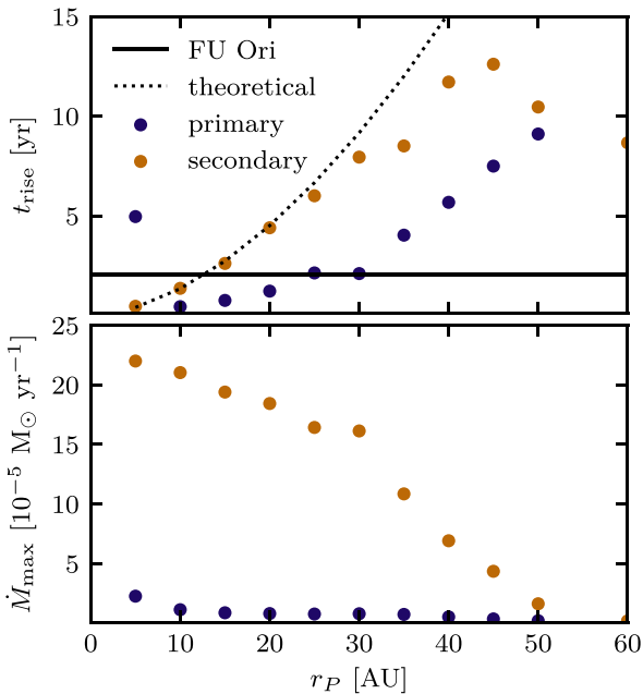
Figure 4. Rise time (top) and maximum mass accretion rate (bottom) for different periastron distances. Dark blue is for the primary star while orange is for the secondary. Horizontal line shows the rise time we calculated for FU Ori from its light curve (see fig. 3 in Hartmann & Kenyon 1996) in the top. The dotted line shows a theoretical estimate for the rise time of the stellar flyby following equation (2).
