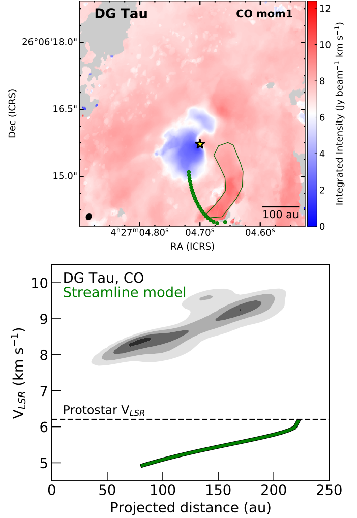
Fig. B.2. Infalling streamline model for the red-shifted southern arc structure (outlined in the green polygon), with the same disk orientation and rotation geometry used for the northern streamer model (Fig. B.1). Top: Streamline model, plotted in green, on top of the moment-1 map of CO, showing the model curvature with this rotation geometry is opposite to the spatial structure of the southern redshifted arc. Bottom: Velocity components of CO taken from inside the green polygon plotted as a function of projected distance from the central young stellar object, with varying levels of kernel density estimation of the velocity plotted as filled contours and contours calculated as in Fig. B.1. The streamline model consistently under-predicts the velocity of the arc structure by \sim 3 km s -1 .
