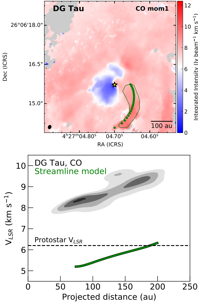
Fig. B.3. Infalling streamline model for the redshifted southern arc structure (outlined in the green polygon), with the same disk orientation but opposite rotation geometry used for Fig. B.2. Top: Streamline model, plotted in green, on top of the moment-1 map of CO, showing the model curvature well matches spatial structure of the southern redshifted arc with the envelope rotation counter-rotating with respect to the disk. Bottom: Velocity components of CO taken from inside the green polygon plotted as a function of projected distance from the central young stellar object, with varying levels of kernel density estimation of the velocity plotted as filled contours and contours calculated as in Fig. B.1. Here, the streamline model also consistently under-predicts the velocity of the arc structure by \sim 3 km s ^{-1} , even though the spatial structure is well matched by the model.
