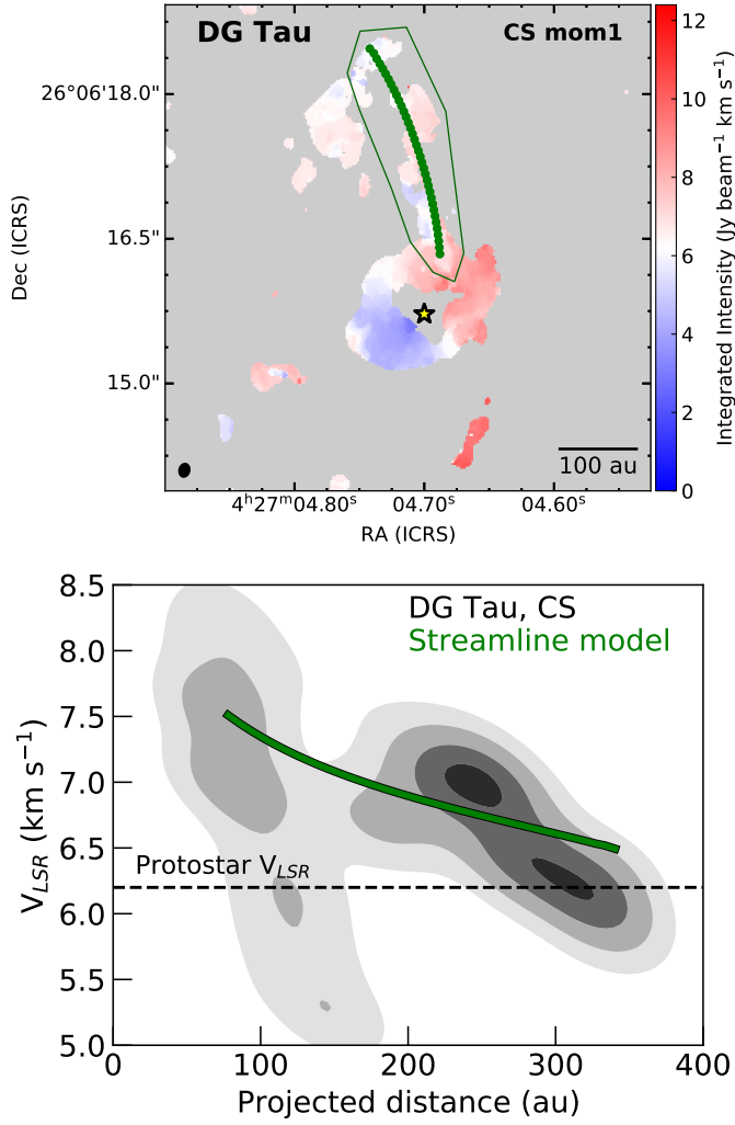
Fig. B.1. Infalling streamline model for the DG Tau streamer. Top: Streamline model, plotted in green, on top of the moment-1 map of CS, spatially matching the observed streamer emission to the north (outlined in the green polygon). Bottom: Velocity components of CS taken from inside the green polygon plotted as a function of projected distance from the central young stellar object, with varying levels of kernel density estimation of the velocity plotted as filled contours. The contours start at 0.5\sigma and progress in steps of 0.5\sigma , where \sigma is from a bivariate normal distribution (see also Pineda et al. 2020). The streamline model, shown in green, describes most of the kinematics of the system in addition to the spatial match shown in the top panel. The main deviation is a small amount of blue-shifted emission in the streamer at a projected distance of \sim 100 -150 au from the central young stellar object.
