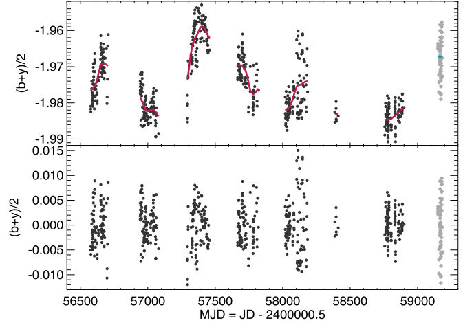
Figure 1. Ground-based APT light curve of \epsilon Eri. Top: Differential (b + y)/2 photometry (in magnitudes) from the T8 (black circles) and T4 (gray diamonds, latest data set) telescopes. The long-term trends are shown in red for the T8 data and in blue for the T4 data. Bottom: The same photometry as above, but with the long-term trends removed. The signature that remains is assumed to be rotational variation and not overall brightening or dimming trends.
