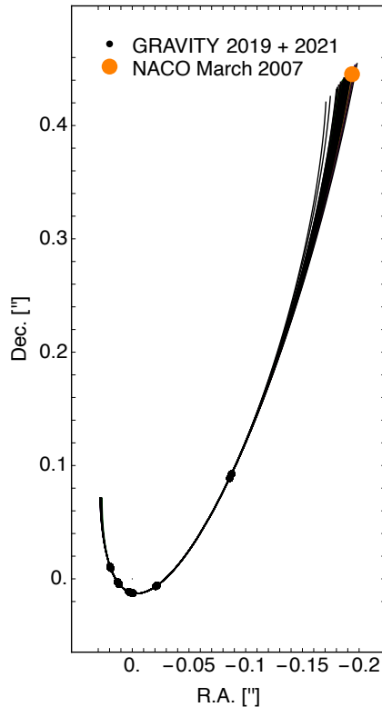
Fig. D.2. Backwards prediction of the GRAVITY data for S29 GRAVITY leads to a position in March 2007 compatible with the position of S29 NACO . The black points show the GRAVITY data from 2021 and 2019. The set of black orbits is obtained by bootstrapping these data and fitting each of these mock data sets. The family of orbits naturally matches the position obtained from NACO (orange disk). The epoch March 2007 was chosen since it is the one used in Gillessen et al. (2009) to define the names of the S-stars.
