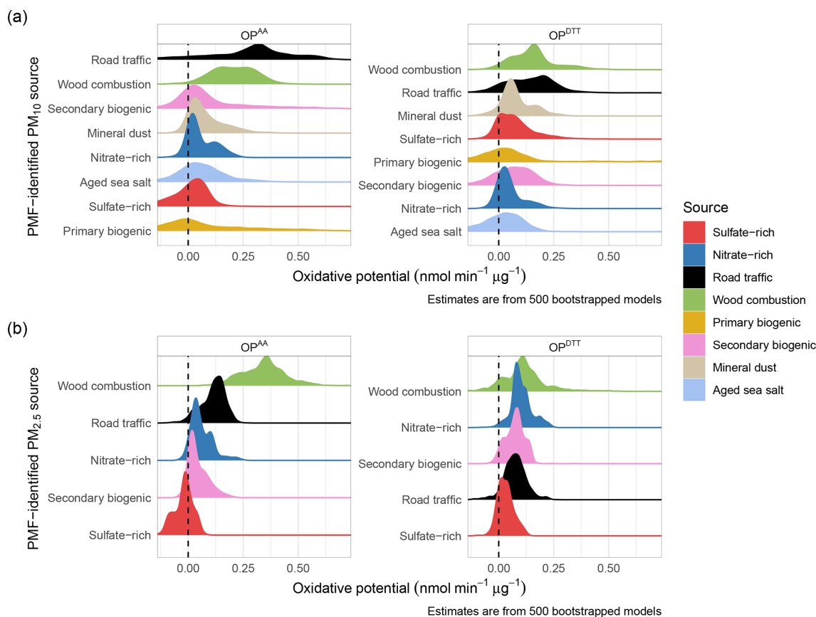
Figure 4. Densities of the intrinsic OP_m^{AA} (a) and OP_m^{DTT} (b) estimates for the eight PM 10 and five PM 2.5 PMF-identified sources. The estimates for all five sites included in the analysis have been aggregated.
