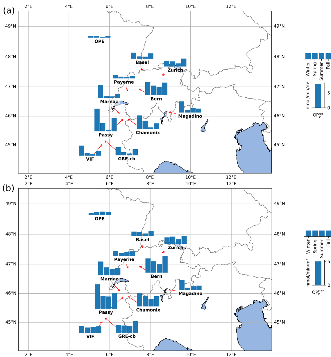
Figure 3. Seasonal OP_V^{AA} (a) and OP_V^{DTT} (b) PM 10 means for the five Swiss sites included in this analysis and the closest six French sites surrounding Switzerland. Data from the French sampling sites are from Weber et al. (2021).
