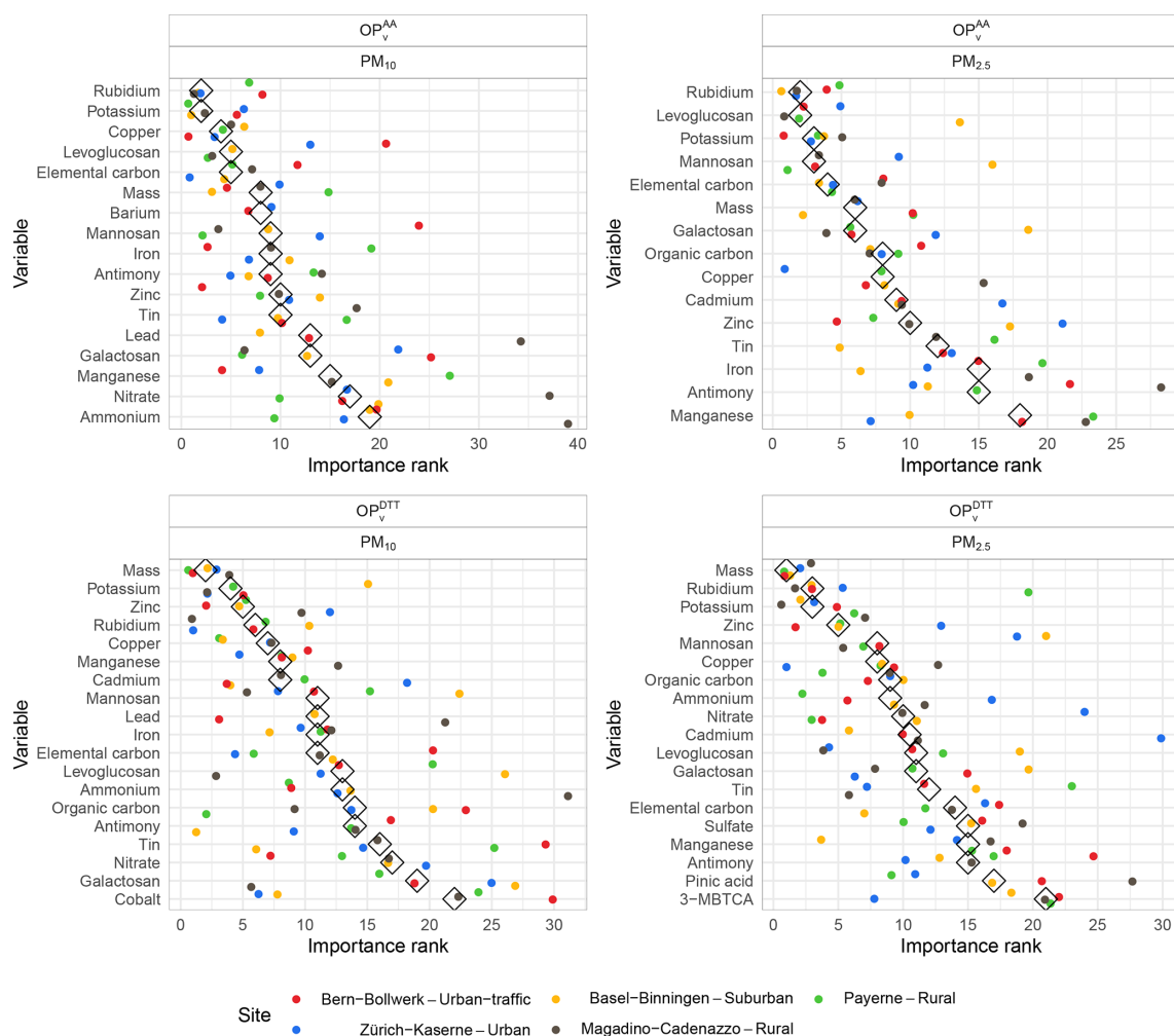
Figure 5. Random forest importance plots of the top independent variables for two OP v assays, two particulate size fractions, and five sampling sites. The large open diamonds represent the variables' medians, and the variables are ordered by median ranking.
