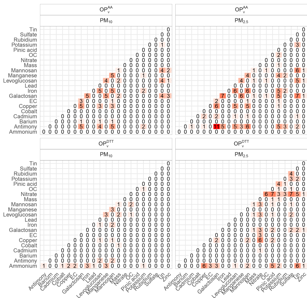
Figure 7. Number of times that a combination of two independent variables for the filtered models was present for PM 10 and PM 2.5 and two OP v assays for five sampling sites.
