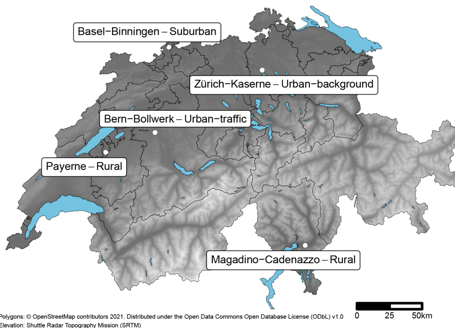
Figure 1. The five sampling sites in Switzerland that were used for PM oxidative potential measurements. The shading indicates the elevation of the terrain and the blue areas show larger lakes and reservoirs. The cantonal boundaries are displayed as lines.
