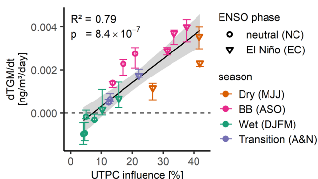
Figure 4. Fit results following Equation 1. There is a significant positive linear relationship between monthly UTPC influence (3-month running average) and monthly CHC dTGM/dt . Error bars give 95% confidence intervals. “2015–2016 El Niño conditions” (EC) from May 2015 to April 2016 and “2014–2015 neutral conditions” (NC) from May 2014 to April 2015. There is a seasonal pattern in fit residuals: dTGM/dt is systematically underestimated in the BB season and overestimated in the wet season. The largest residuals fall into the dry season.
