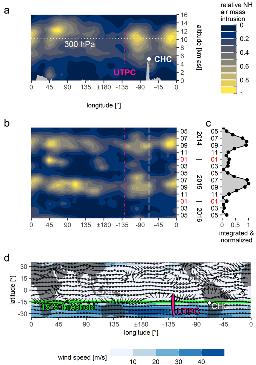
Figure 5. Pathways and seasonality of Northern Hemisphere (NH) air mass intrusion as estimated by 21-day HYSPLIT forward trajectories: (a) altitude profile of the relative magnitude of NH air mass intrusion into the Southern Hemisphere (SH) tropics. Magnitude of NH air mass intrusion estimated by counting how many HYSPLIT forward trajectories emitted in the NH crossed the threshold latitude 15°S (compare to green line in (d)) during their 21-day runtime (all forward trajectories between February 2014 and August 2016). NH air mass intrusion occurs preferentially in the mid-to-upper troposphere (UT), approximately between 6 km and 14 km asl. Three preferred longitudinal bands for NH air mass intrusion emerge, centered around the longitudes 60°, −90°, and −10°. Terrain altitude from the HYSPLIT digital elevation model at the 15°S intersection is shown in gray. (b) Temporal evolution of NH air mass intrusion at 15°S (at altitudes above mixing height as taken from GDAS1, see Section 2.4.3). NH air mass intrusion shows a marked seasonality, with the strongest magnitude between July and September. For the longitudes 100°–170°, NH air mass intrusion appears somewhat enhanced in 2015, as compared to 2014. (c) Estimated temporal evolution of NH air mass intrusion into the global SH tropical UT, obtained by zonal integration of panel (b) and min-max normalization. (d) NCEP/NCAR reanalysis wind vector fields at 300 hPa (compare to dotted line in (a)) between June 2015 and October 2015 reveal fast eastward transport in the SH tropical UT. Wind vector length is independent from wind speed, which is color-coded instead. Pink arc shows definition of the UTPC. The 15°S threshold latitude 15°S where NH air mass intrusion was estimated (for panels (a–c)) is shown as green line.
