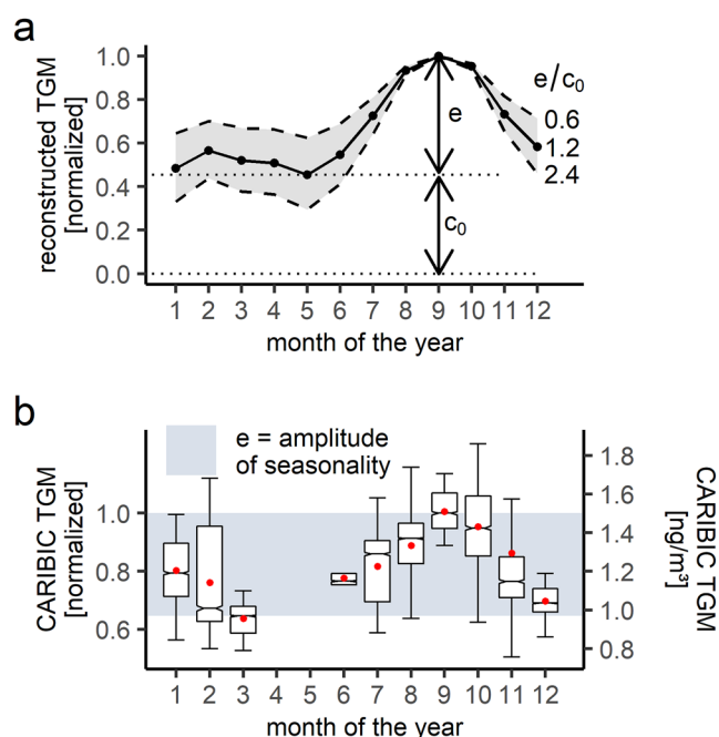
Figure 7. Reconstructed total gaseous mercury (TGM) seasonality and comparison to aircraft data on upper tropospheric TGM. (a) Reconstructed TGM seasonality in the upper tropospheric pacific channel (UTPC), based on Chacaltaya TGM under the hypothesis that UTPC TGM seasonality is driven by interhemispheric exchange. The magnitude of seasonality is expressed as ratio between amplitude of seasonal variation ( e ) and constant baseline concentration ( c_0 ). Shaded area based on the 95% confidence interval of e/c_0 (0.6–2.4). (b) Measured upper tropospheric TGM seasonality east of the UTPC, based on CARIBIC flights between 2005 and 2016 (latitudes: 25°S–5°S, longitudes: –50° to –30°; for comparison, the UTPC was defined at ~–125°). Blue area: estimated amplitude of CARIBIC TGM seasonality, defined as difference between highest and lowest monthly median (September and March, respectively). Normalized values (left axis) obtained by division through the highest monthly median (September). Box plot outliers ( <Q1 - 1.5 \cdot IQR or > Q3 + 1.5 \cdot IQR ) are not shown. Red dots show mean values. Reconstructed (a) and measured (b) seasonality agree well, peaking simultaneously during September. While the amplitude of reconstructed seasonal variation appears higher than measured, the difference is not statistically significant ( \alpha = 0.05 ), considering the e/c_0 95% confidence interval (shaded area in (a)).
