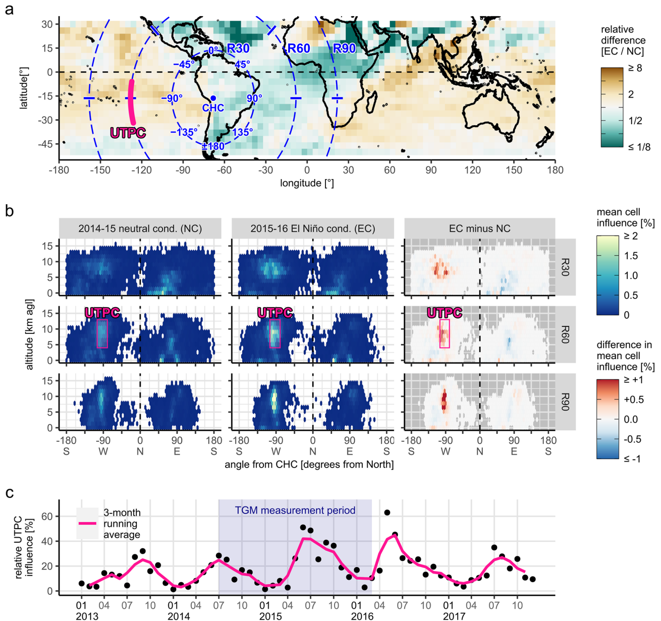
Figure 3. Westwards shift in Chacaltaya (CHC) air mass origin in 2015–2016 as characterized by 21-day HYSPLIT back trajectories. (a) Relative difference in source region influence between “2014–2015 neutral conditions” (NC, here May 2014 to April 2015) and “2015–2016 El Niño conditions” (EC, here May 2015 to April 2016), defined as the total number of HYSPLIT trajectories crossing a grid cell during EC divided by the total number of HYSPLIT back trajectories crossing the same grid cell during NC. The dashed circles (R30, R60, and R90) show three cylindrical cross-cuts corresponding to radii of 30, 60, and 90 geographical lat/lon degrees from CHC, respectively. Note that points on individual circles are not equidistant to CHC due to the spherical shape of the Earth. Blue numbers show angle from CHC in angular degrees (North = 0°). The definition of the UTPC is given as pink arc (see also (b)). (b) Altitude profiles of CHC air mass origin during NC, EC, and their difference, at selected radii from CHC (dashed circles in (a)). These altitude profiles are based on “cylindrical slices”, by which we reduce each HYSPLIT back trajectory to points on cylindrical cross-cut surfaces (see Section 2.4.2, Figure 1). The mean cell influence was defined as the percentage of all back trajectories emitted from CHC that crossed the respective cell on the cylindrical surface during their 21-day run duration. Most El Niño-anomalies in westerly transport can be narrowed down to a relatively narrow mid-to-upper tropospheric “channel”, which we define as “upper tropospheric pacific channel” (UTPC, pink arc in (a)). (c) Evolution of relative UTPC influence, defined as percentage of all emitted 21-day back trajectories that passed through the UTPC before reaching CHC. The influence of the UTPC varies seasonally and was amplified in 2015–2016.
