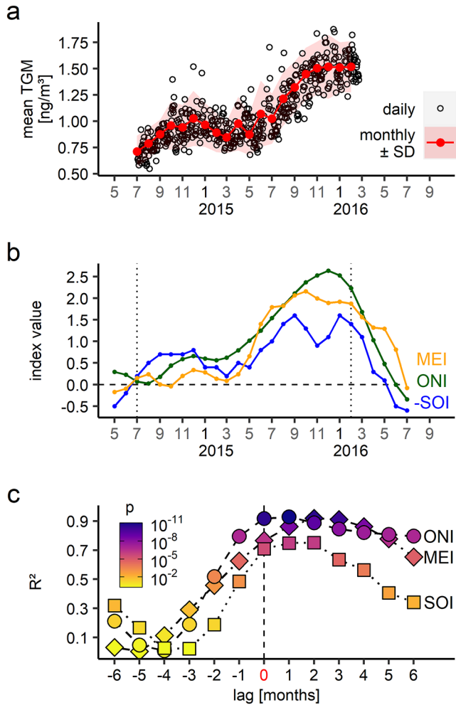
Figure 2. Chacaltaya (CHC) TGM observations and the onset of the 2015–2016 El Niño. (a) Steep increase of CHC TGM in 2015. Daily (monthly) arithmetic averages in black (red). Red shaded area: monthly average + \pm 1 standard deviation. (b) Similar steep increase of ENSO indices (ONI, MEI, SOI) during the same months as in (a). SOI was multiplied by -1 to facilitate comparison between indices. The vertical dashed lines show the TGM measurement period. (c) CHC TGM lags behind ENSO indices by 1–2 months. We estimated the most likely time lag by computing R^2 (Pearson) between monthly TGM (a) and ENSO indices (b) for several lags. Positive (negative) lags mean that monthly TGM reacts after (before) the respective index.
