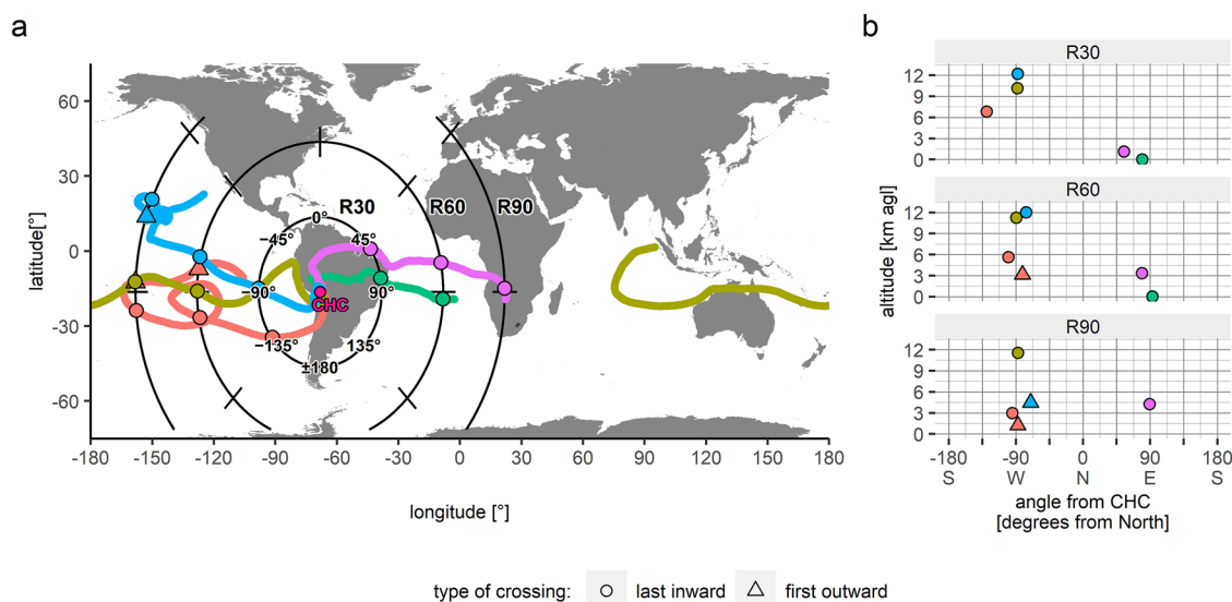
Figure 1. Illustration of the “cylindrical slices” approach used to characterize 3-D air mass origin. Five back trajectories were chosen as an example. (a) The black circles marked R30, R60, and R90 show three cylindrical slices corresponding to radii of 30, 60, and 90 geographical lat/lon degrees from CHC, respectively. Note that, given the spherical shape of the Earth, points on individual circles are not equidistant to CHC. Numbers show the angle from CHC in degrees (North = 0°). Circles and triangles indicate where a back trajectory crossed the respective cylindrical slice. (b) Back-trajectories in their representation on the cylindrical slices R30, R60, and R90. Each point on each surface indicates where the respective cylindrical slice was crossed by a back trajectory. Each trajectory can be represented by up to two different points on each cylindrical surface, corresponding to the last inward crossing (moving toward CHC) and the first outward crossing (moving away from CHC) of the cylindrical surface. While a trajectory can cross the same slice more than twice, this is very rare.
