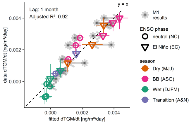
Figure 6. Significant improvement of dTGM/dt prediction by the inclusion of interhemispheric exchange. Fit based on Equation 3, assuming a lag of 1 month between TGM in the UTPC and upper tropospheric interhemispheric transport (hence UTPC TGM peaking in September). Error bars show 95% confidence intervals. “2015–2016 El Niño conditions” (EC) from May 2015 to April 2016, “2014–2015 neutral conditions” (NC) from May 2014 to April 2015. Dashed line gives the 1:1 reference. Stars show fitted values as obtained by the fit following Equation 1 (M1). Arrows indicate how fitted values changed from M1 to the best fit following Equation 3 (M2), thus visualizing the effect of including the seasonality of NH air mass intrusion into the fit. In contrast to M1, there is no seasonal pattern in the residuals of fit M2.
