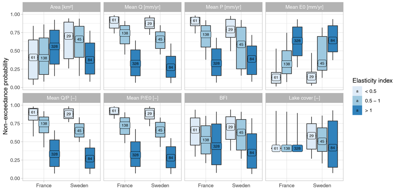
Figure 7. Distribution of hydroclimatic characteristics according to three classes of the elasticity index ( \epsilon_2 ) in Eq. (2). The numbers within each boxplot describe the number of catchments. The boxes are delimited by quantiles 0.25 and 0.75; whiskers by quantiles 0.1 and 0.9.
