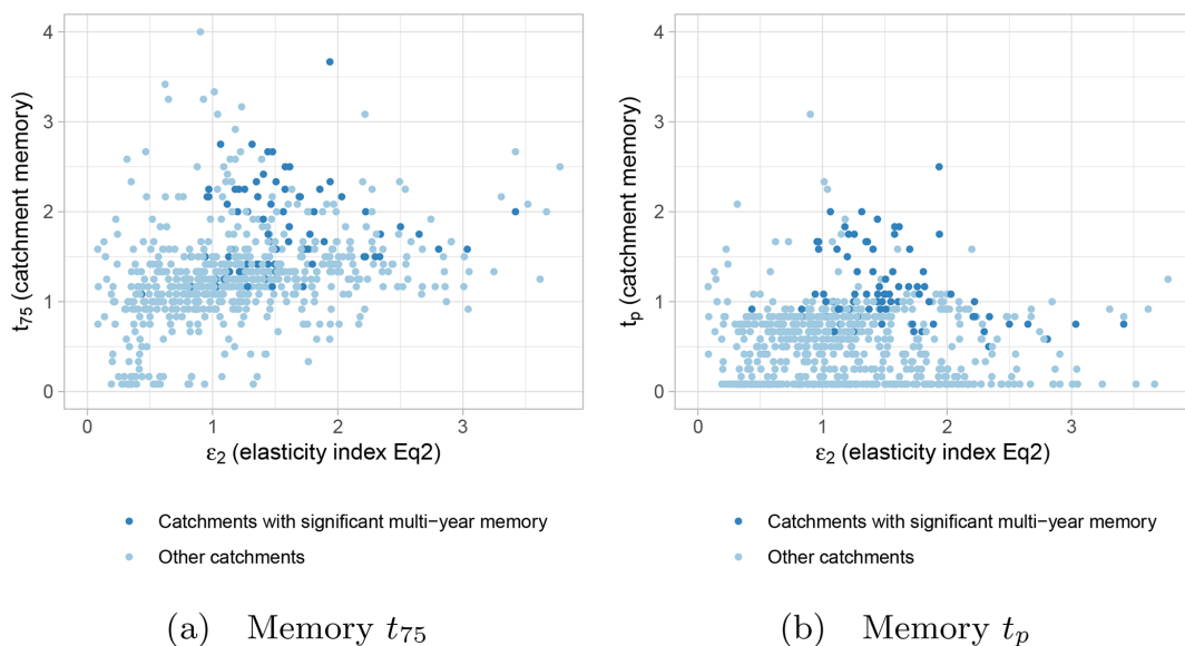
Figure A1. Relation between elasticity index ( \epsilon_2 ) of Eq. (2) and catchment memory assessed by t_{75} and t_p .
