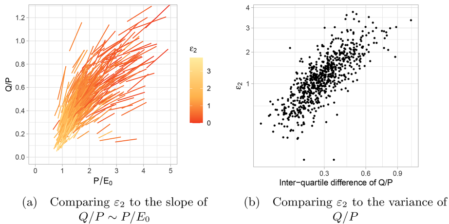
Figure 8. Comparison of the elasticity index ( \epsilon_2 , Eq. 2) with the slope in the linear relation between Q/P and P/E_0 (a), and with inter-quartile differences of Q/P values (b). Slopes can be visualized for each catchment through the segments. Segments are drawn between the two points defined by the first and third quartiles of these two ratios. A square root transformation is applied to both axes.
