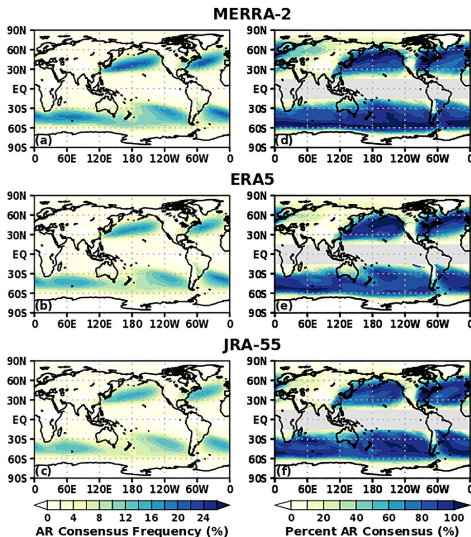
Figure 5. The frequency of occurrence of consensus ARs, with at least half of the global ARDTs detecting an AR, in (a) MERRA-2, (b) ERA5, and (c) JRA55 and the frequency of occurrence of consensus ARs as a percentage of the ensemble mean AR frequency in (d) MERRA-2, (e) ERA5, and (f) JRA55.
