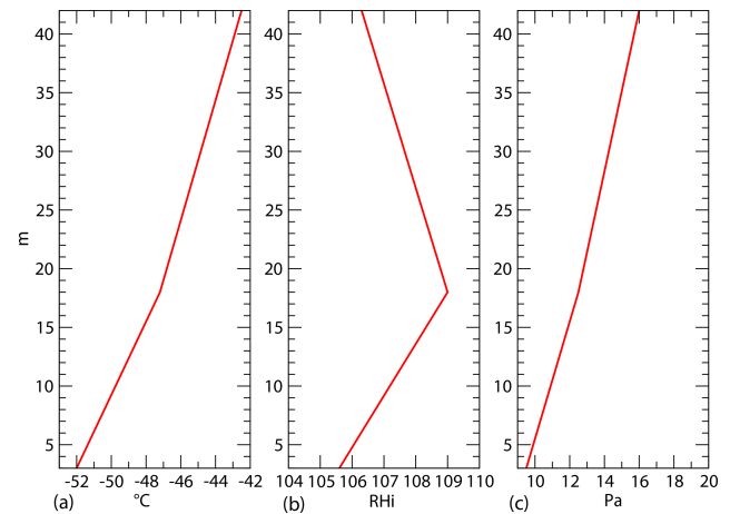
Figure 9. Annual mean vertical profile of temperature (a), RHi (b) and PPW (c) for observations made from 2018 to 2020.
