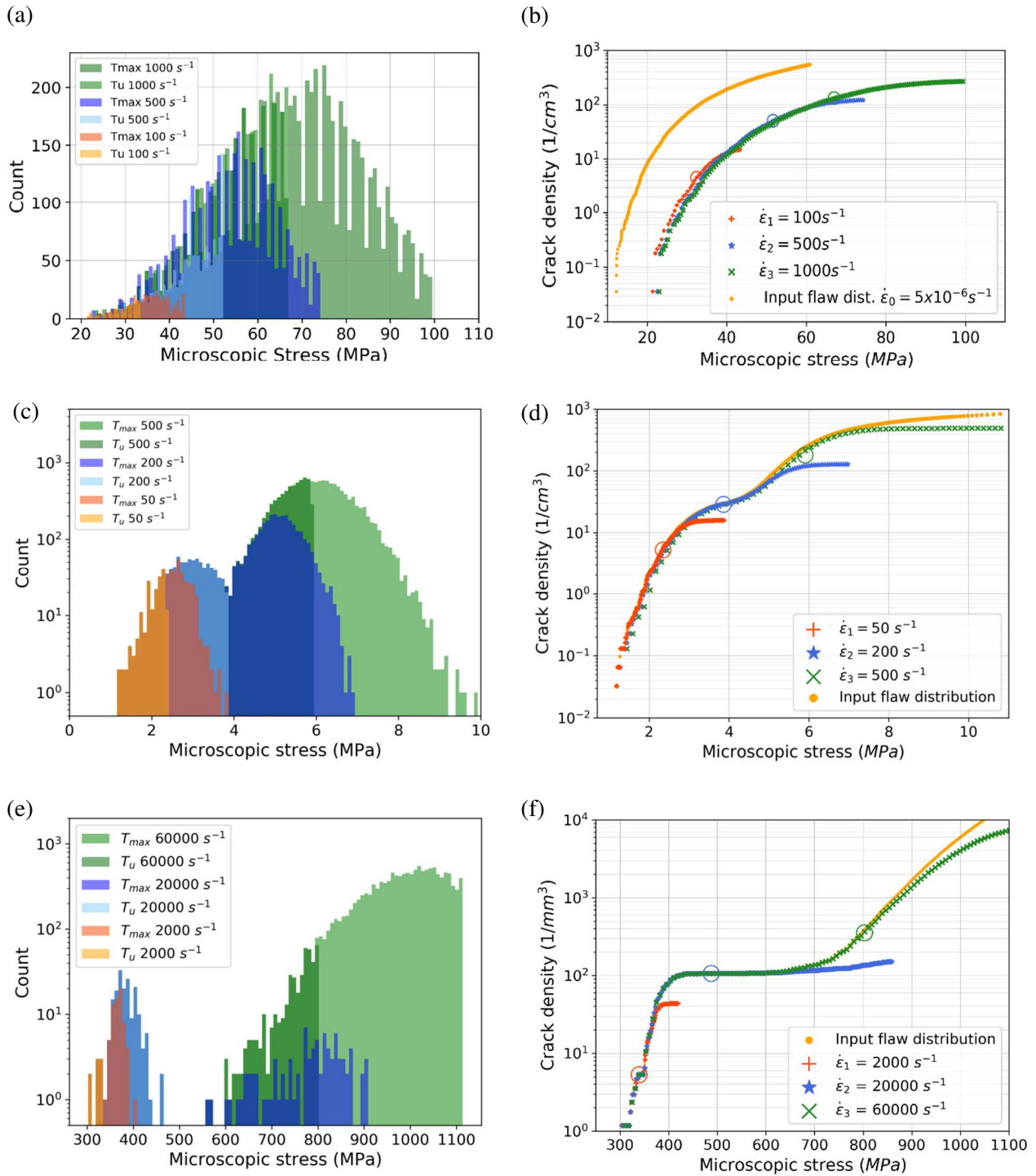
Figure 11. Results of discrete numerical calculations. (a-b) UHPC, (c-d) Porous ice, (e-f) SiC ceramic with size-controlled porosity. (a, c, e) Overlapped histograms of the number of activated flaws at T_u (time at which the ultimate strength is reached) and T_{max} (time at which the whole volume is obscured) for three levels of strain rates. (b, d, f). Evolution of the crack density as function of the microscopic stress for three levels of strain rates. The crack density level corresponding to the time at which the ultimate strength is reached is circled for each loading rate.
