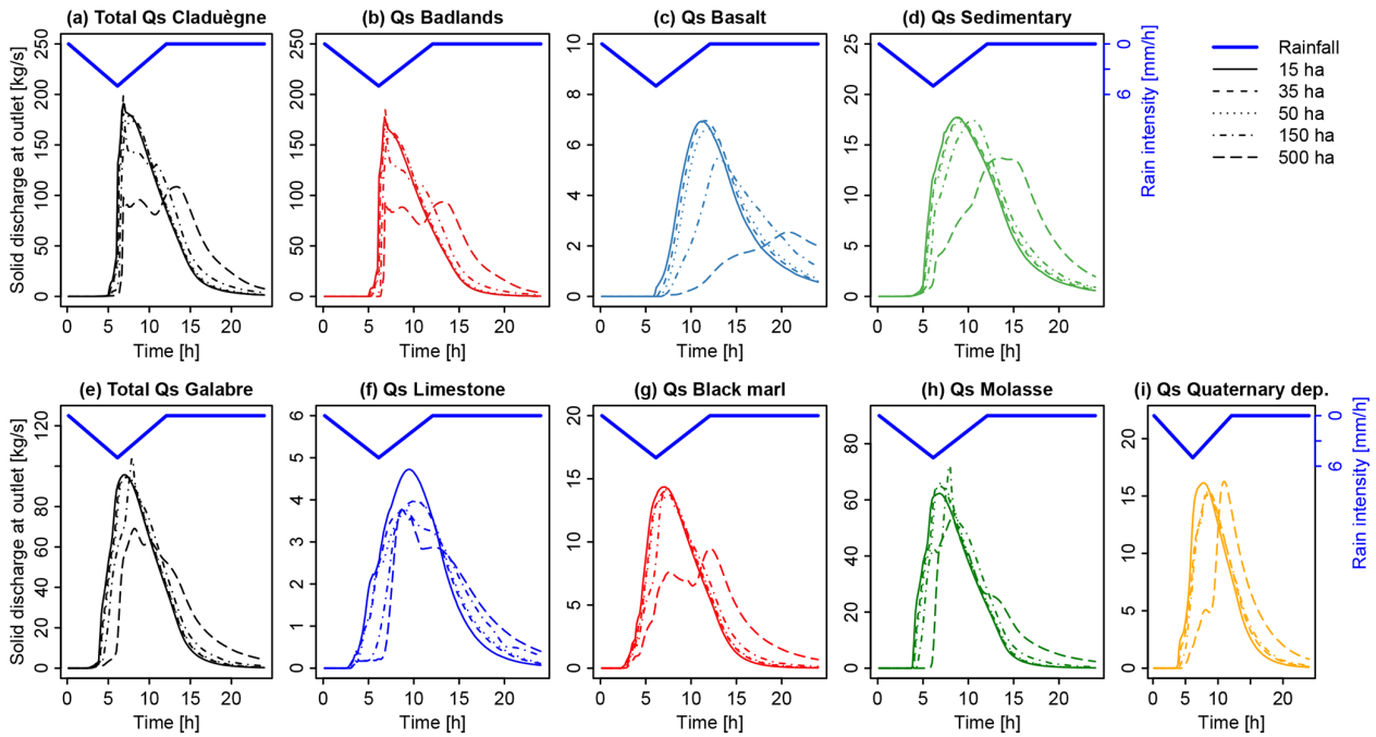
Figure 6. Simulated sedigraphs for total suspended solid discharge ( Q_s ) and for each source in the two catchments when different values are used for the threshold of contributing drainage area (CDA) to define the river network.
