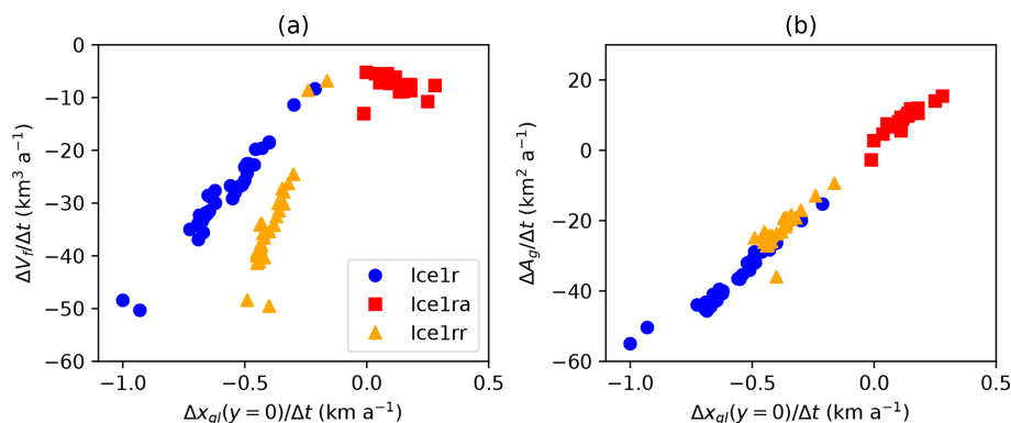
Figure 5. Rates of change in midchannel grounding line position x_{gl}(y=0) plotted against rates of change in volume above flotation V_f (a) and grounded area A_g (b). For all three of the Ice1r, Ice1ra, and Ice1rr experiments each point \left(\frac{\Delta x_{gl}(y=0)}{\Delta t}, \frac{\Delta V_f}{\Delta t}\right) lies close to a straight line, as do the points \left(\frac{\Delta x_{gl}(y=0)}{\Delta t}, \frac{\Delta A_g}{\Delta t}\right) , despite the considerable variation between models.
