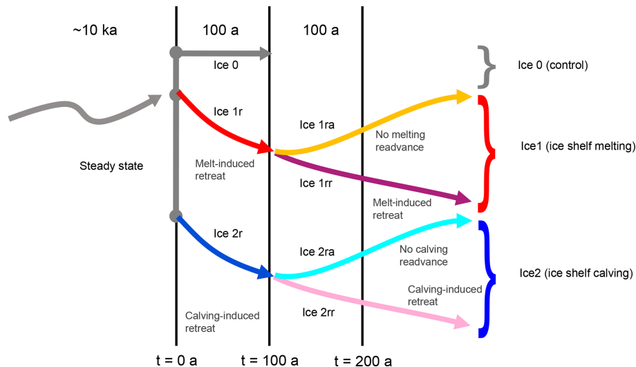
Figure 1. Relationship between the MISIMIP+ Ice0, Ice1, and Ice2 experiments. An upward sloping curve indicates an advancing grounding line, a downward sloping curve a retreating grounding line. All three experiments start from a common steady state. The Ice0 experiment provides a control for the Ice1 and Ice2 experiments, which induce retreat with ice shelf melting or calving respectively for 100 a. Later stages of the experiments remove or continue the melting or calving.
