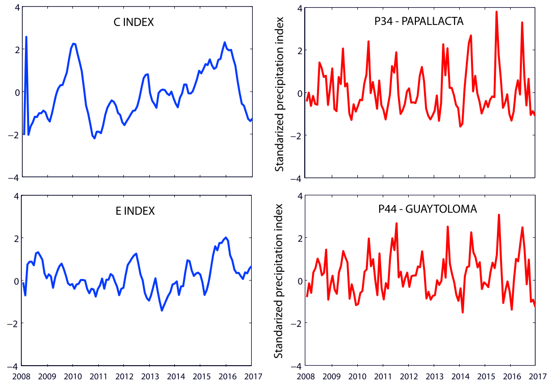
Figure A1. Modes of variability associated with the ENSO phenomenon (blue curves): (1) the increase in the central Pacific (C Index) variability that is associated with stronger cold events, and (2) the reduction in the eastern Pacific (E Index) variability within the cold/moderate warm regime. The standardized precipitation of the two rain gauge stations (P34 and P44) of our study basin in the period of analysis (red curves). ENSO = El Niño–Southern Oscillation.
