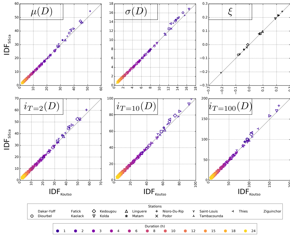
Figure 6. Comparison between IDF_{SiSca} and IDF_{Koutso} in calibration mode. Top panels: location parameter – \mu(D) [ mm\ h^{-1} ]; scale parameter – \sigma(D) [ mm\ h^{-1} ]; and shape parameter – \xi [–]. Bottom panels: return levels – i_T [ mm\ h^{-1} ] – obtained for different return periods T ranging from 2 to 100 years displayed.
