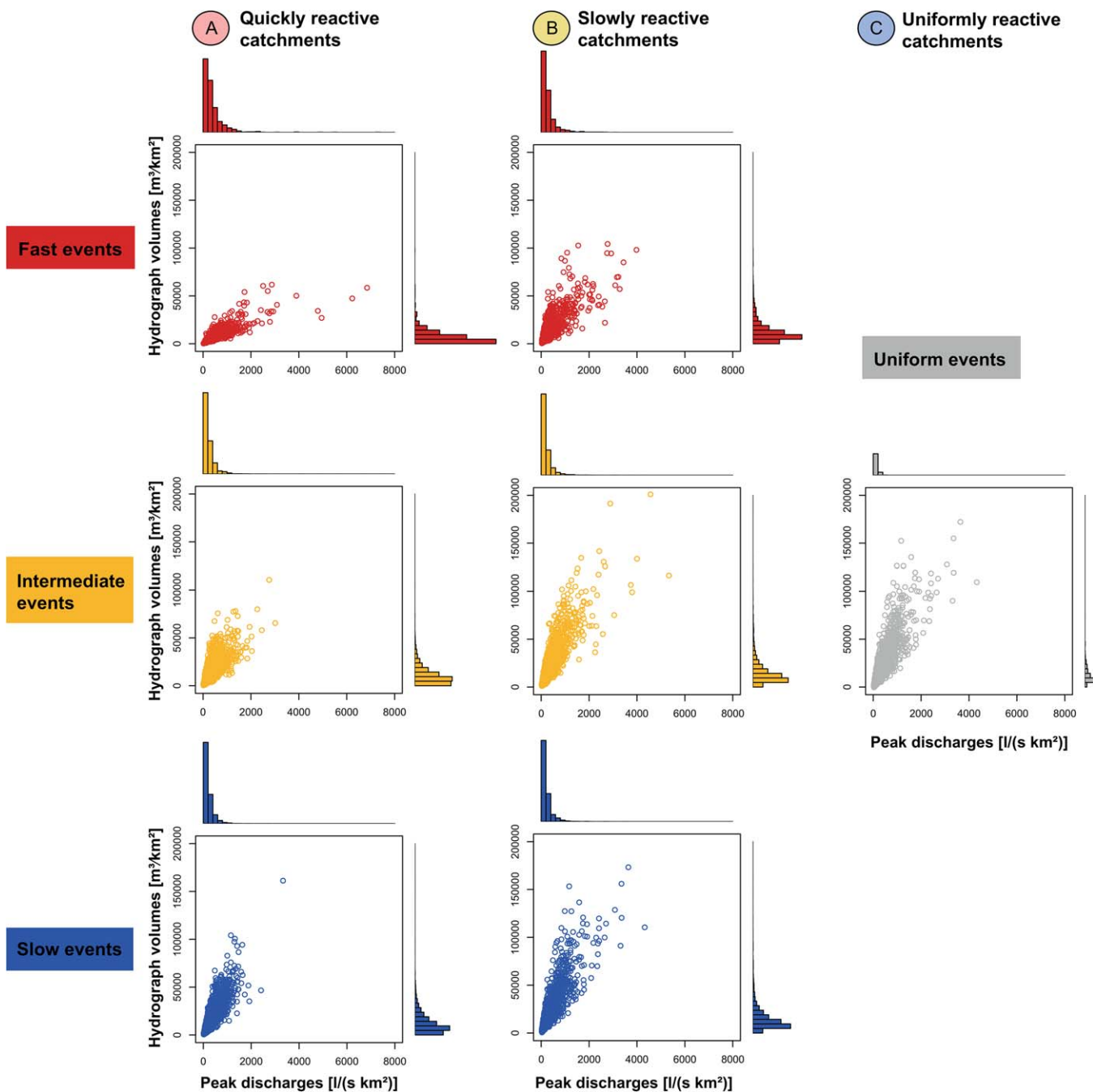
Figure 10. Specific peak discharges ( l/(s km^2) ) and hydrograph volumes ( m^3/km^2 ) for the event types in the three reactivity regions ((a) quickly reactive, (b) slowly reactive, and (c) uniformly reactive). The two variables are jointly displayed as a scatter plot and separately in a histogram. The scales of the histograms and scatter-plots are the same across all event types and reactivity regions.
