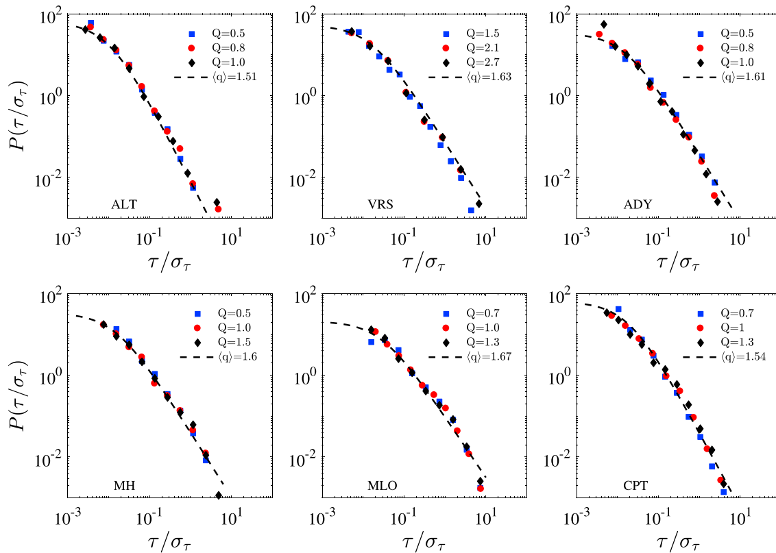
Figure 5. Log-log plot of PDF P(\tau/\sigma_\tau) for the normalized IOT extracted from Hg^0 data recorded at different latitudes and different threshold Q . Dashed line is the averaged q exponential fit (equation (3)).
