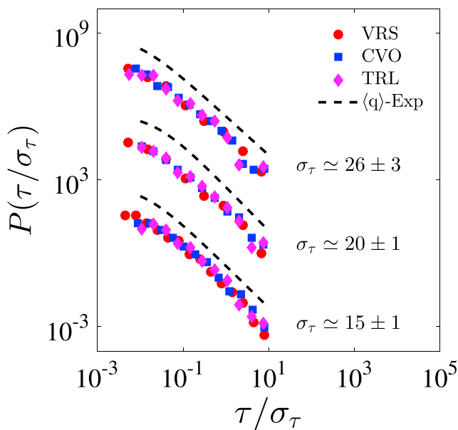
Figure 6. Log-log plot of PDFs P(\tau/\sigma_\tau) for the normalized IOT obtained at three different sites and at three different thresholds Q : VRS 81^\circ N , 17^\circ W , CVO, and TRL 72^\circ S , 2^\circ E ). The plots have been arbitrarily shifted vertically for clarity. For VRS, Q=0.6, 1.3, 1.5 ; CVO, Q=0.7, 0.9, 1 ; and TRL, Q=0.9, 1.1, 1.3 . For these thresholds all the data possess the same \sigma_\tau . Dashed lines are the q exponential fit (equation (3)).
