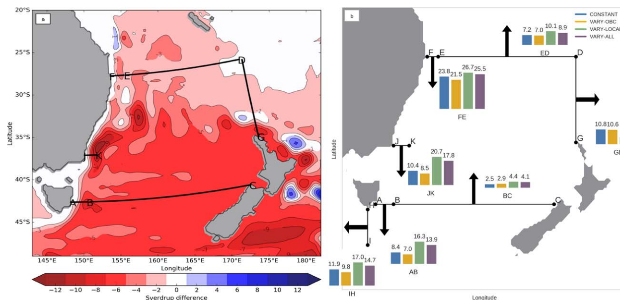
Figure 5. (a) Time-mean barotropic streamfunction difference between VARY-LOCAL and CONSTANT (integration taken eastward from Australia down to 1,945 m; contours every 2 Sv), red (blue) indicates areas of enhanced (reduced) transport when local surface forcing is introduced. (b) Comparison of depth-integrated transport (Sv) to 1,945 m between CONSTANT (blue), VARY-OBC (yellow), VARY-LOCAL (green), and VARY-ALL (lavender). The section end points are the same as Figure 3, with the addition of points J (150.1°E, 37.1°S) and K (151.7°E, 37.1°S).
