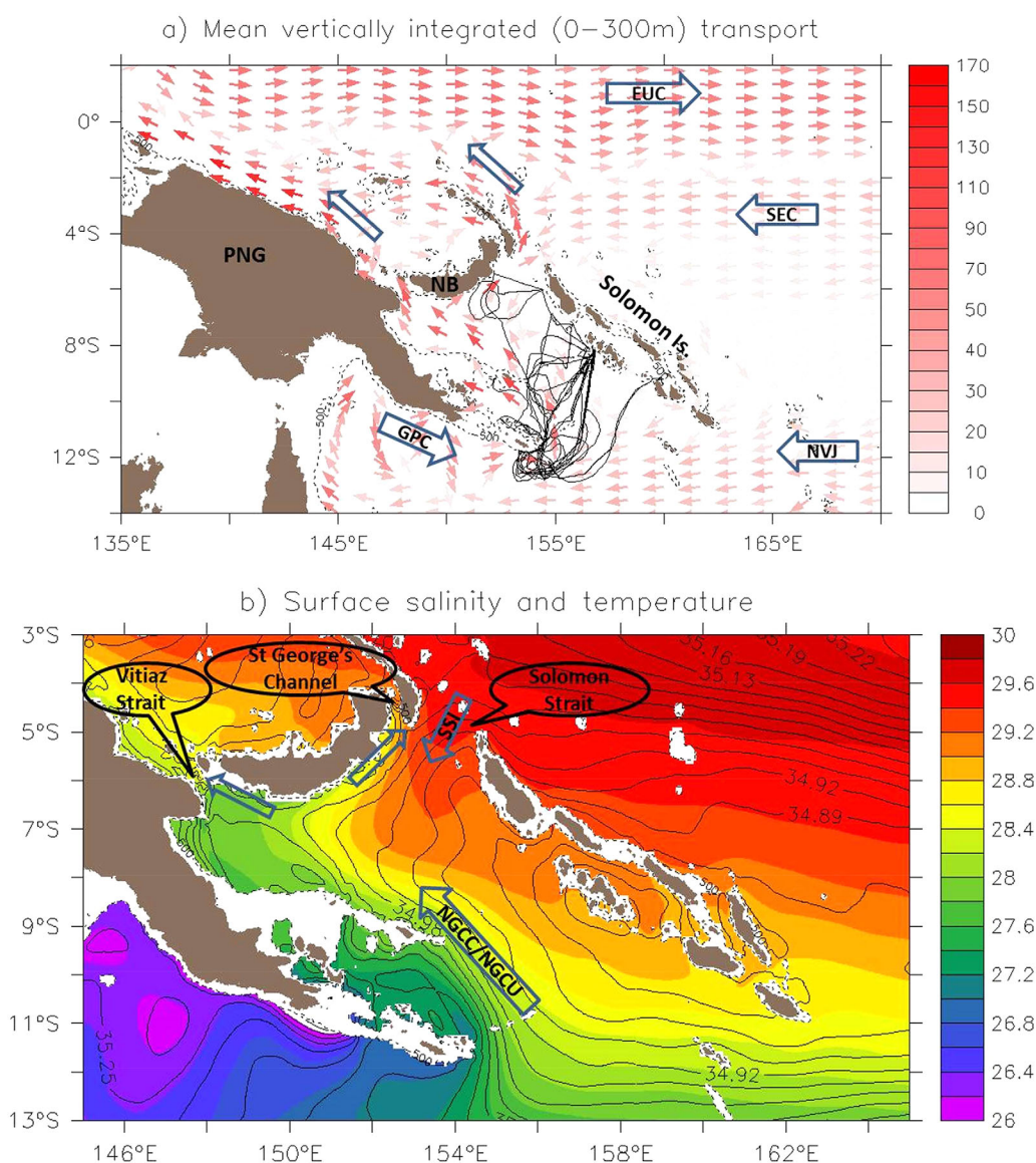
Figure 1. (a) Mean vertically integrated (0–300 m) transport (in \text{m}^2 \text{s}^{-1} ) in the southwestern tropical Pacific computed from the Drakkar ORCA12 simulation. Superimposed are the 11 glider tracks sampling the Solomon Sea circulation during the 2007–2011 period. The main currents surrounding the Solomon Sea are shown in Figure 1a: the Gulf of Papua Current (GPC), the North Vanuatu Jet (NVJ), the South Equatorial Current (SEC), and the Equatorial Undercurrent (EUC). PNG stands for Papua New Guinea and NB for New Britain. (b) A zoom in on the Solomon Sea of the mean sea-surface salinity (SSS in contours) and temperature (SST in color, ^{\circ}\text{C} ) from the Drakkar ORCA12 simulation. Arrows stand for the main Solomon Sea currents which are the New Guinea Coastal Current (NGCC), New Guinea Coastal Undercurrent (NGCU), and the Solomon Strait Inflow (SSI). The dashed line represents the 500 m isobath. Additional arrows in Figures 1a and 1b show direction of mean flow.
