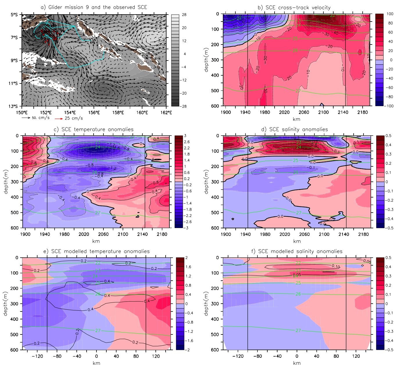
Figure 7. Same as Figure 5 for the stationary cyclonic eddy SCE9 of mission #9.
