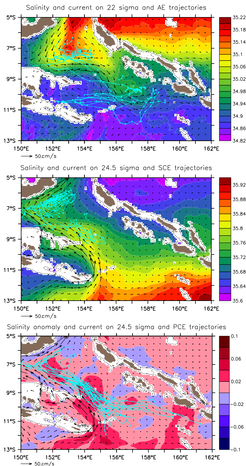
Figure 12. (a) Salinity and current fields at the 22 sigma level density averaged over the time where AEs are present. AEs trajectories are superimposed in light blue. (b) Salinity and current fields at the 24.5 sigma level density averaged over the time where SCEs are present. SCEs trajectories are superimposed in light blue. (c) Salinity anomaly (relative to the reference low-frequency field) and current fields at the 24.5 sigma level density averaged over the time where PCEs are present. PCEs trajectories are superimposed in light blue.
