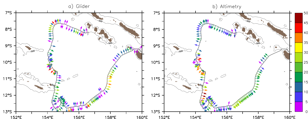
Figure 3. Absolute cross-track geostrophic current (in \text{cm s}^{-1} ) for the glider mission #2 estimated (a) from glider averaged over the 0–150 m depth and (b) from altimetry.
