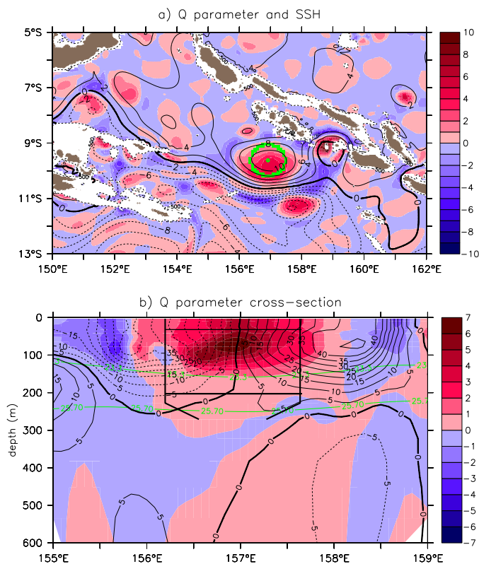
Figure 8. (a) Horizontal distribution of the Q parameter (shading, 10^{-9} \text{ s}^{-2} ) estimated from the model exhibiting an AE centered at 156.9^\circ\text{E} , 9.6^\circ\text{S} (green point). The green circle delineates the eddy radius. Superimposed in contour is the SSH field. (b) Depth/longitude section of the Q parameter (shading, 10^{-9} \text{ s}^{-2} ) at the location of AE. The thick black lines delineate its horizontal extension function of depth defined by the max swirl velocity and its vertical extension from the NL parameter defined to 1. The thin black line locates the mixed layer depth. The velocity section ( \text{cm s}^{-1} ) is in black contours, and the density ( \text{kg m}^{-3} ) of SW and UTW are in green contours.
