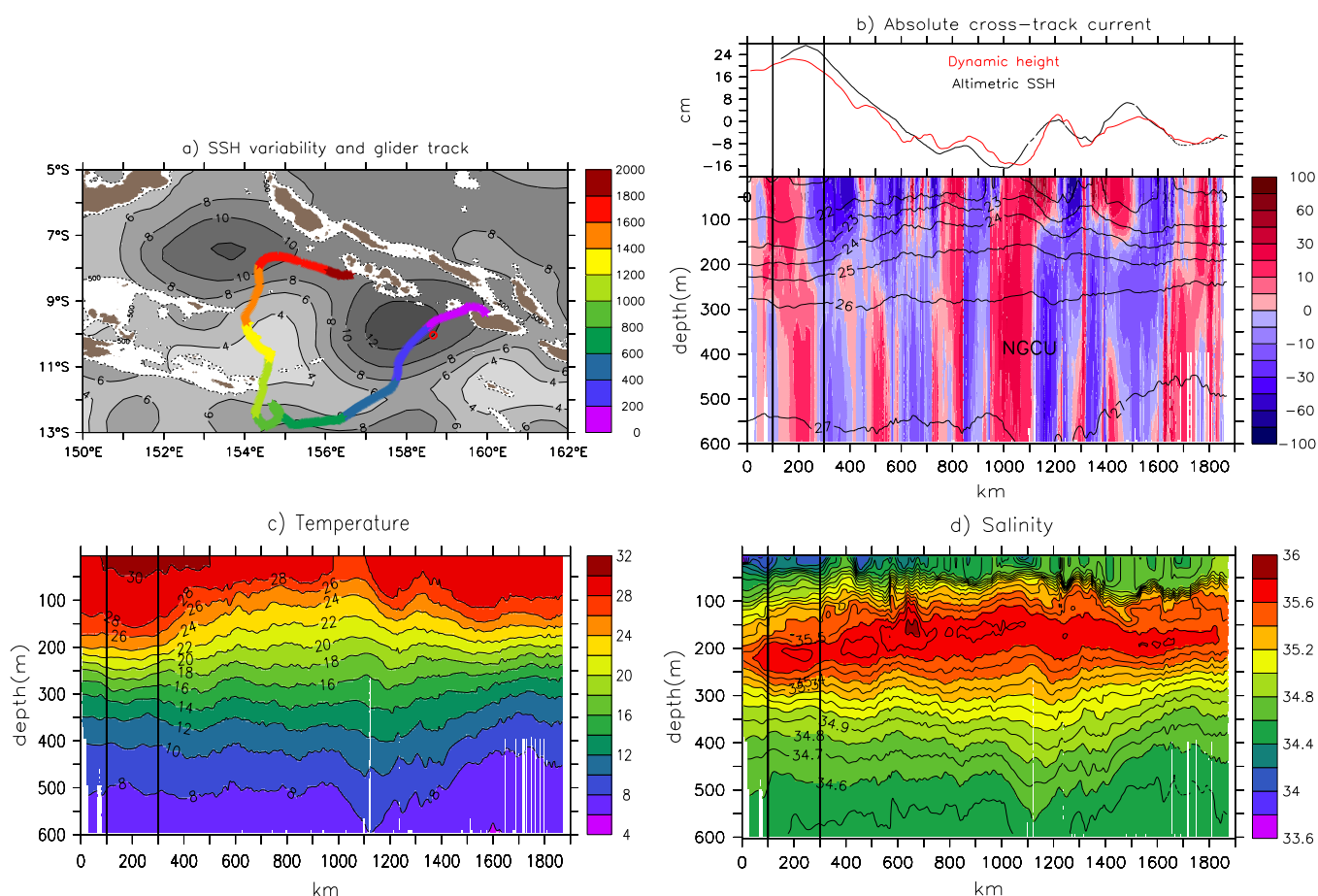
Figure 2. Description of the glider mission #2. (a) Distance (in km, colors) covered from the beginning of the glider's mission. Grey shading shows the standard deviation of SSH (in cm) during the 5 months of the glider mission. (b)–(d) Vertical profiles along the glider track of absolute cross-track geostrophic velocity ( \text{cm s}^{-1} , positive to the right of the track), temperature ( ^{\circ}\text{C} ), and salinity sampled by the glider, respectively. On top of Figure 2b, are shown the dynamic height inferred from glider data (in red) and the SSH from altimetry (in black), in cm. Thick black lines in Figures 2b–2d delineate the anticyclonic eddy describes in section 3.1.
