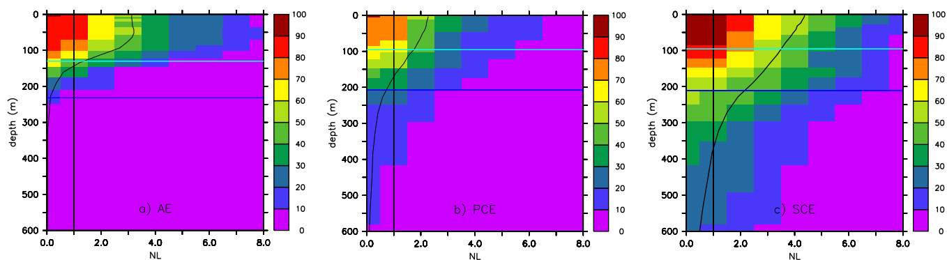
Figure 9. (a) Vertical profile of the nonlinear parameter (NL) averaged for all AEs (Thick black line). In shading is the periodogram of NL showing the distribution of cumulative number of eddies from high to small NL in percentage of the total number of eddies. The thin vertical line is for NL = 1 . The cyan (blue) horizontal lines are for the 23.3 (25.7) sigma level that define SW (UTW), respectively. (b) Same as Figure 9a for PCEs and (c) same as Figure 9a for SCEs.
