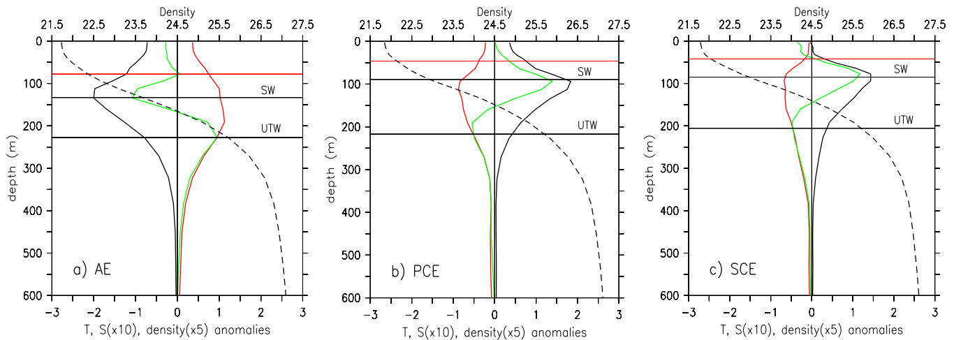
Figure 10. Mean temperature (red, °C), salinity (green, psu), and density (thick black, \text{kg m}^{-3} ) anomalies within eddies as a function of depth for (a) AEs, (b) PCEs, and (c) SCEs. The corresponding mean density profile of the reference fields (i.e., section 3.2) is shown as a dashed line. Horizontal black lines delineate the Surface Water (SW) and Upper Thermocline Water (UTW). The red line indicates the mixed layer depth. The x axis on top is for density ( \text{kg m}^{-3} ) whereas x axis on bottom is for anomalies of temperature, Salinity ( \times 10 ), and density ( \times 5 ).
