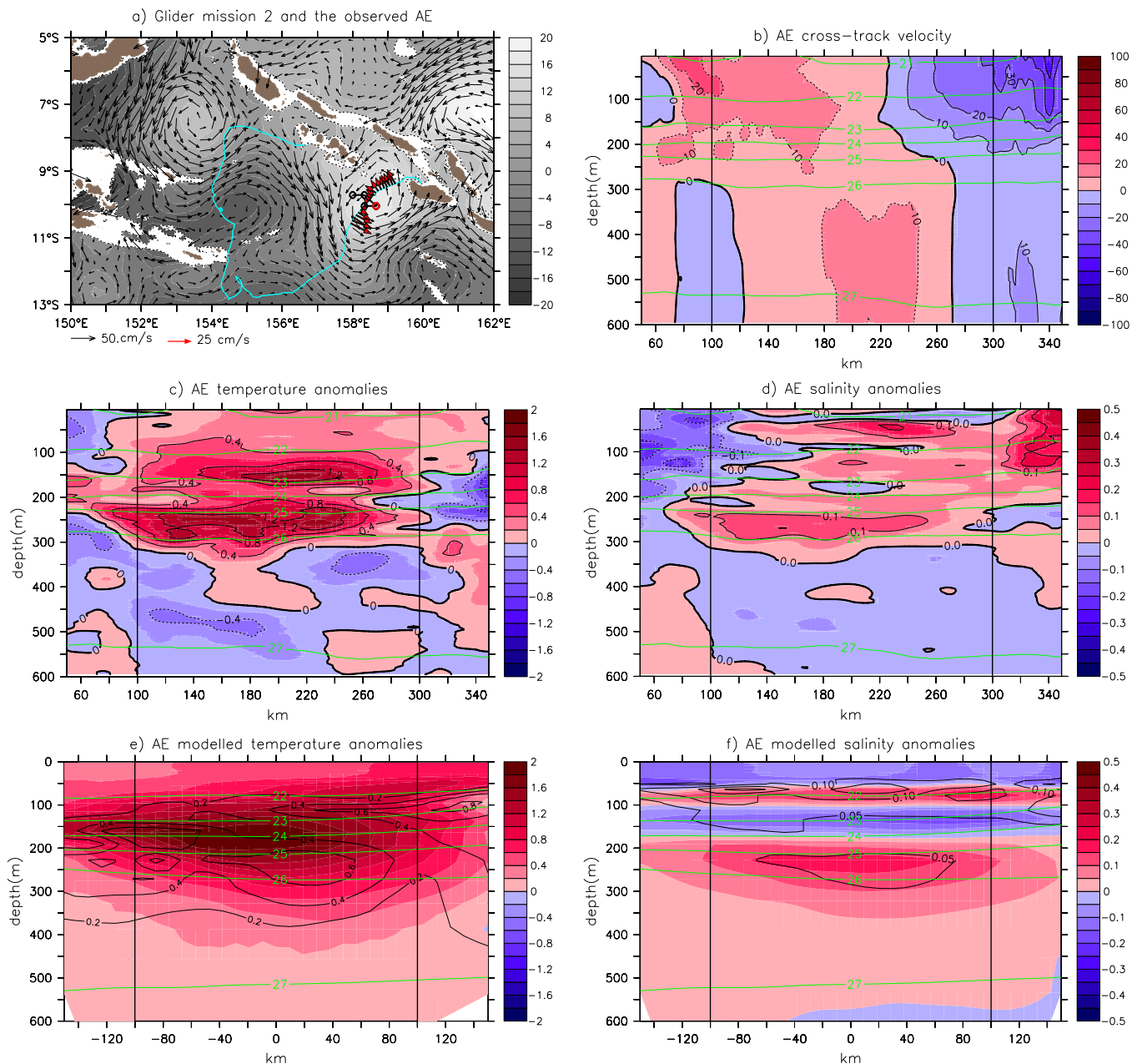
Figure 5. Signature of the anticyclonic eddy AE2 observed by the glider along its track during mission 2. (a) The dot line is the trajectory of AE2 detected on the altimetric maps, and the red dot is the location of AE2 when it has been sampled by the glider. Grey shading and black arrows show the altimetric SSH field (cm) and the corresponding geostrophic velocity field, respectively, on 12 March 2008 when A2 was sampled. The glider track is in cyan whereas the red arrows correspond to the absolute cross-track geostrophic velocity in the surface layer computed from the glider data. (b) Vertical section of the glider cross-track absolute geostrophic velocity (cm s -1 ) across AE2. (c) and (d) Vertical section of temperature (°C) and salinity anomalies, respectively. (e) and (f) are the composite signatures of modeled AEs for temperature (°C), and salinity, respectively (see text for details). The composite structures are in shading, and the corresponding standard deviation is in black contours. Density (kg m -3 ) are in green contours. The black vertical lines delineate the eddy.
