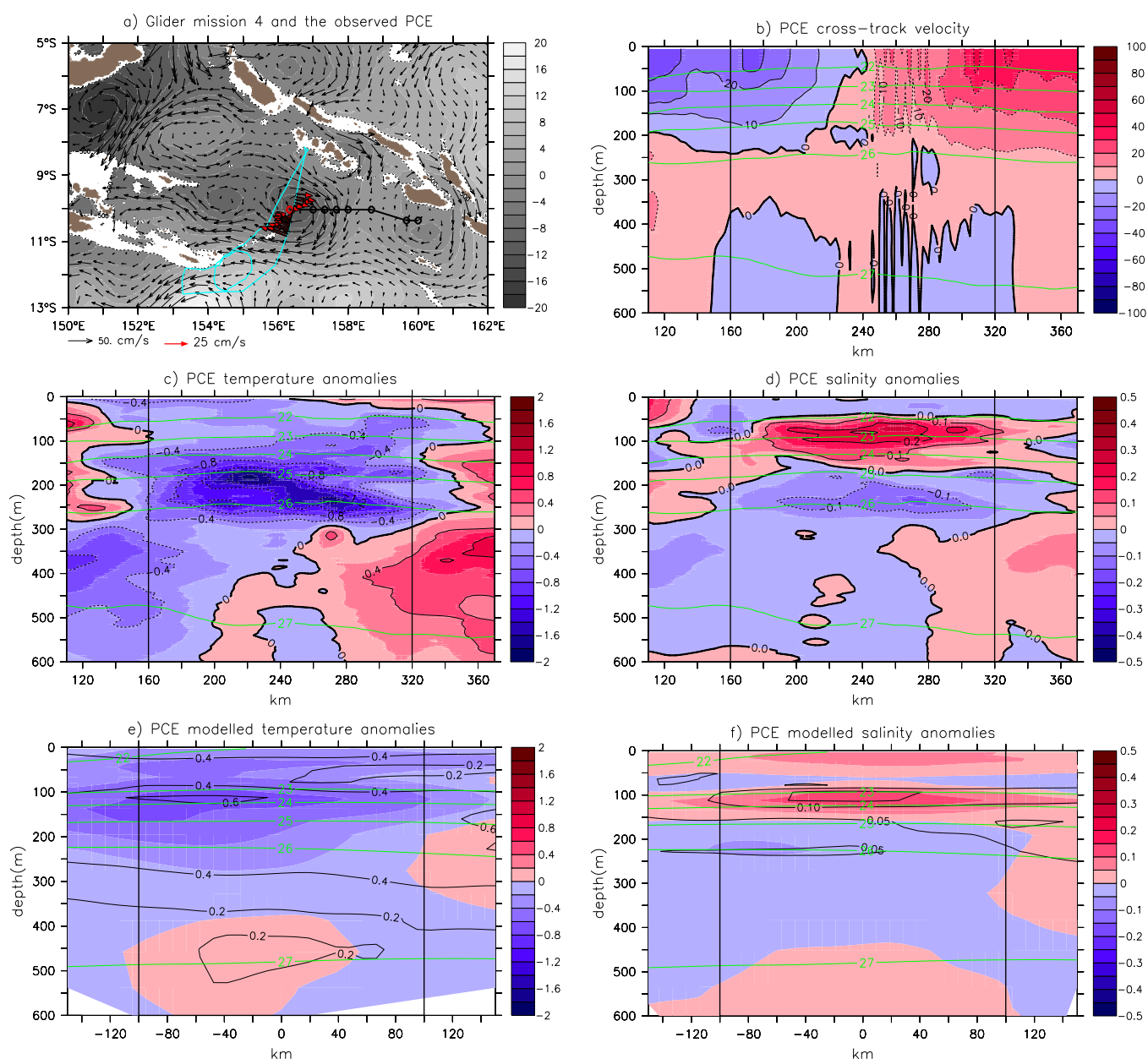
Figure 6. Same as Figure 5 for the propagating cyclonic eddy PCE4 of mission #4.
