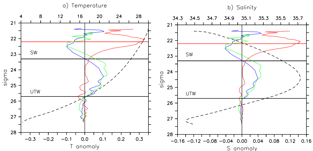
Figure 11. (a) Temperature (°C) and (b) salinity anomalies as a function of sigma levels for AEs (red), PCEs (blue), and SCEs (green). The thick-dashed line shows the mean (a) temperature and (b) salinity profile in the Solomon Sea. Horizontal black lines delineate the two main water masses: Surface Water (SW) and Upper Thermocline Water (UTW). The horizontal red line indicates the mean density at the mixed layer depth.
