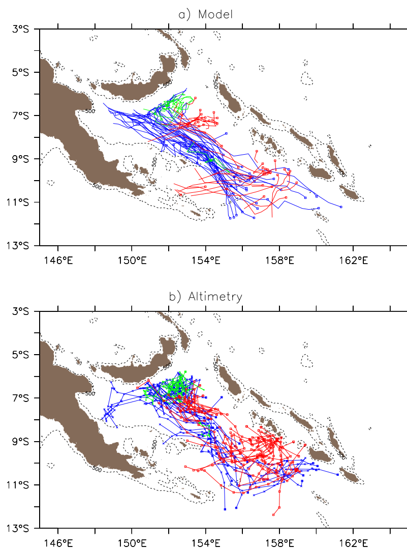
Figure 4. Distribution of the propagating CEs (in blue, defined by propagating distances > 300 km), stationary CEs (in green, defined by a life span > 5 weeks and by propagating distances < 200 km), and AEs (in red) for (a) the model and (b) altimetry.
