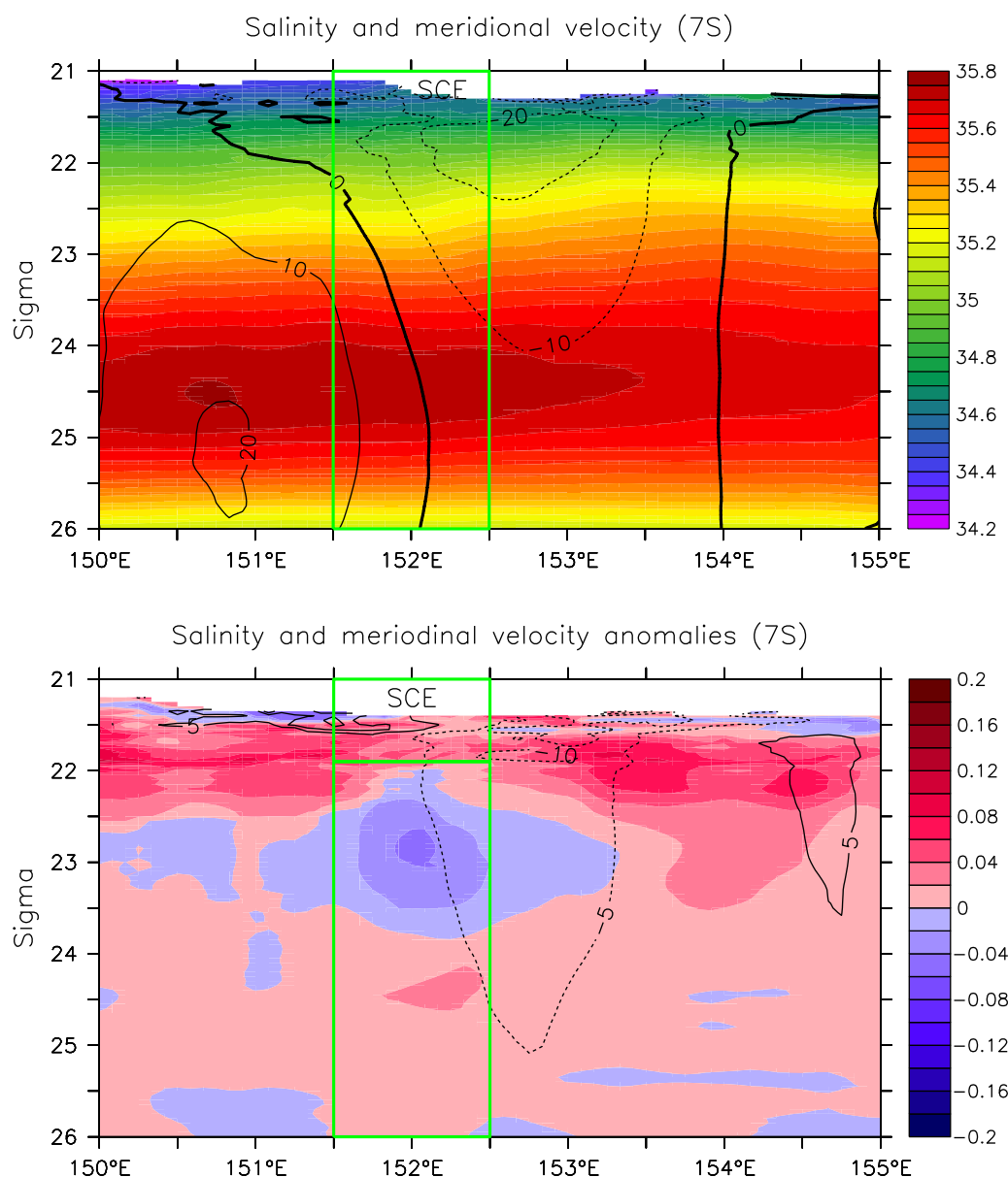
Figure 13. (a) Longitude/sigma density section at 7°S of salinity (psu, shading) and meridional velocity ( \text{cm s}^{-1} , contour) averaged over the time where SCEs are present. (b) Same as Figure 13a but for salinity and meridional velocity anomalies relative to the reference low-frequency field. The green lines delineate the mean position and mixed layer sigma density level of SCEs.
