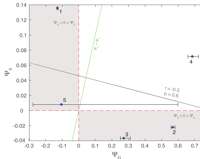
Figure 5. Hysteresis metric calculated from seismic ( \Psi_S ) and geophone ( \Psi_G ) data for each transport event (1–5). The red dashed lines are \Psi_S = 0 and \Psi_G = 0 , and the gray regions demark areas where the direction of hysteresis is reversed between seismic and geophone data (clockwise versus counterclockwise). The green line indicates \Psi_S = \Psi_G , and the gray line shows regression between \Psi_S and \Psi_G ( r = -0.3 , p = 0.6 ). The error bars on \Psi_G represent the maximum range of values corrected for possible temporary sediment storage effects (equation (3)).
