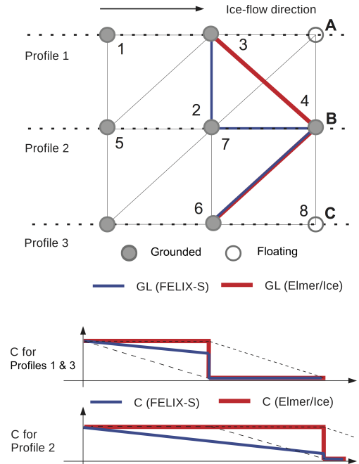
Figure 1. A schematic of the different basal boundary masking schemes used by FELIX-S and Elmer/Ice and their impact on the definition of the MISIMIP3d basal friction coefficient ( C(x, y) is assumed uniform beneath grounded ice for illustrative purposes. For floating ice, C(x, y) = 0 ). Circles denote the nodes at the ice–bed interface, defining the basal finite element faces (triangular and quadrilateral for FELIX-S and Elmer/Ice, respectively); open circles denote floating nodes for which z(x, y, t) > b(x, y) ; and solid circles denote grounded nodes for which z(x, y, t) = b(x, y) and -\sigma_{nn} > P_w . Numbers 1–8 identify triangular element faces of FELIX-S and letters A–C identify specific nodes common to both models. As discussed in Sect. 6, the different masking schemes lead to the different grounding-line positions and also to the different nodal values of C along profiles 1–3. The C profiles based on DI for Elmer/Ice (heavy red line) and FELIX-S profiles (heavy blue line) are shown, as are the corresponding Elmer/Ice FF (black dashed) and LG (black dotted) profiles.
