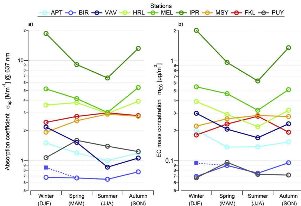
Fig. 4. Seasonal patterns of the geometric mean values for a) absorption coefficients and b) EC mass concentrations. The square marker for Birkenes indicates the geometric mean of all winter data excluding December 2011, which was an outlier from a meteorological point of view, whereas the corresponding circular marker includes December 2011.
