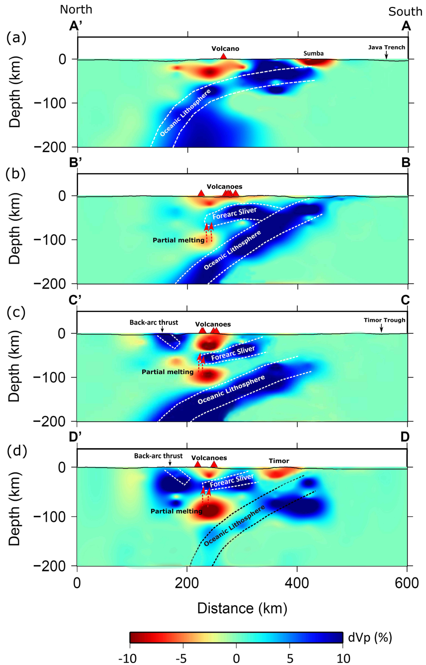
Figure 3. Vertical sections for the V_p model along (a) A-A', (b) B-B', (c) C-C', and (d) D-D'. Models are plotted with a perturbation scale of \pm 10\% . The locations of vertical sections are shown in Figure 1.
