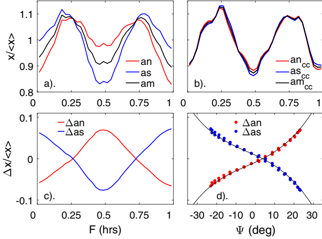
Fig. 12. (a) The observed variations of the geomagnetic indices with fraction of year, F , shown as means in 36 equal-sized bins as a fraction of their overall mean: (red) an(F)/\langle an \rangle_{\text{all}} ; (blue) as(F)/\langle as \rangle_{\text{all}} ; and (black) am(F)/\langle am \rangle_{\text{all}} . (b) The variations after correction for conductivity effects: (red) an_{\text{cc}}(F)/\langle an_{\text{cc}} \rangle_{\text{all}} ; (blue) as_{\text{cc}}(F)/\langle as_{\text{cc}} \rangle_{\text{all}} ; and (black) am_{\text{cc}}(F)/\langle am_{\text{cc}} \rangle_{\text{all}} . The deviations of an and as from am , (red) \Delta an = an - am , (blue) \Delta as = as - am , which for these variations with F are taken to be due to conductivity effects alone. (c) The variations of (red points) \Delta an and (blue points) \Delta as as a function of the mean dipole tilt angle, \psi for the same F -UT. The black lines in (d) are 4th-order polynomial fits to the points that are used to correct an to an_{\text{cc}} and as to as_{\text{cc}} , using equations (6) and (9), respectively.
