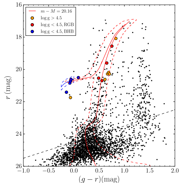
Figure 3. Colour–magnitude diagram of the central 7 arcmin of Aqu 2. The red line is a PARSEC isochrone with [\text{Fe}/\text{H}] = -1.8 , age 12 Gyr and m-M = 20.16 . The blue dashed contour marks the selection area of BHB stars (with five stars) used to constrain the distance to Aqu 2 and the dashed red line delineates the isochrone mask. The dashed black line corresponds to g = 24.5 , which is the limiting magnitude that we use when determining structural parameters of Aqu 2. Large filled circles mark stars with measured spectra, in orange we show likely dwarf stars with \log(g) > 4 (representing contamination), and in blue and red we show giants with \log(g) < 4 (likely BHB and RGB stars, respectively).
