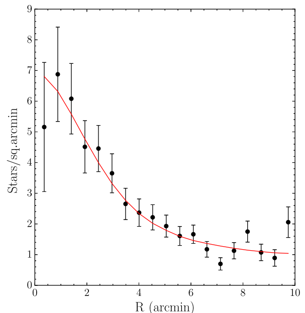
Figure 5. Radial number density profile of Aqu 2 as probed by the stars inside the isochrone mask shown in Fig. 2. The red line shows the best-fitting model, which is formed by a flat background and an elliptical Plummer profile with r_h = 5.1 arcmin and 1 - b/a = 0.39
