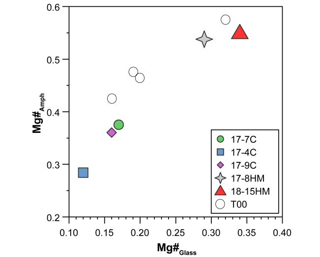
Figure 5. Positive correlation between Mg# of amphiboles and glasses suggesting conditions close to equilibrium. T00: data from Tiepolo et al. (2000).
