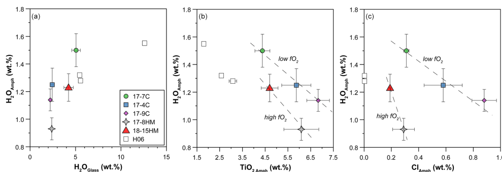
Figure 7. (a) Relation between \text{H}_2\text{O} contents (wt %) in amphiboles and quenched melt. Correlation between \text{H}_2\text{O} content (wt %) in amphibole and its \text{TiO}_2 (b) and Cl (c) contents (wt %). In (c) two separated correlations are visible based on the f\text{O}_2 of the system (dashed lines are a visual guide). H06: data from Hauri et al. (2006).
