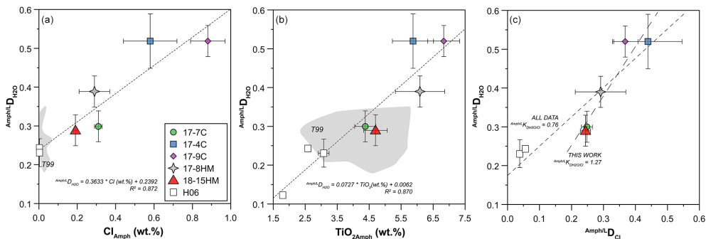
Figure 8. Correlation between \text{Amph}/L\text{D}_{\text{H}_2\text{O}} and Cl (a) and \text{TiO}_2 (b) contents (wt %) in amphibole. H06: data from Hauri et al. (2006); T99: data from Tiepolo (1999). The diagram in (c) shows the correlation between \text{Amph}/L\text{D}_{\text{H}_2\text{O}} and \text{Amph}/L\text{D}_{\text{Cl}} , giving their exchange coefficient ( \text{Amph}/L\text{K}_{\text{DH}_2\text{O}/\text{Cl}} ). \text{Amph}/L\text{K}_{\text{DH}_2\text{O}/\text{Cl}} obtained from this work is 1.27, although it becomes lower than unity considering all data (this study and data from Hauri et al., 2006).
