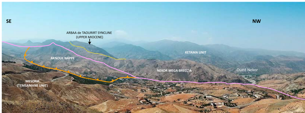
Figure 6. Panoramic view illustrating the Nekor megabreccia and the structural relationship between the Ketama Unit, the Higher nappes (Aknoul), and the Mesorif (South Tamsamani).
