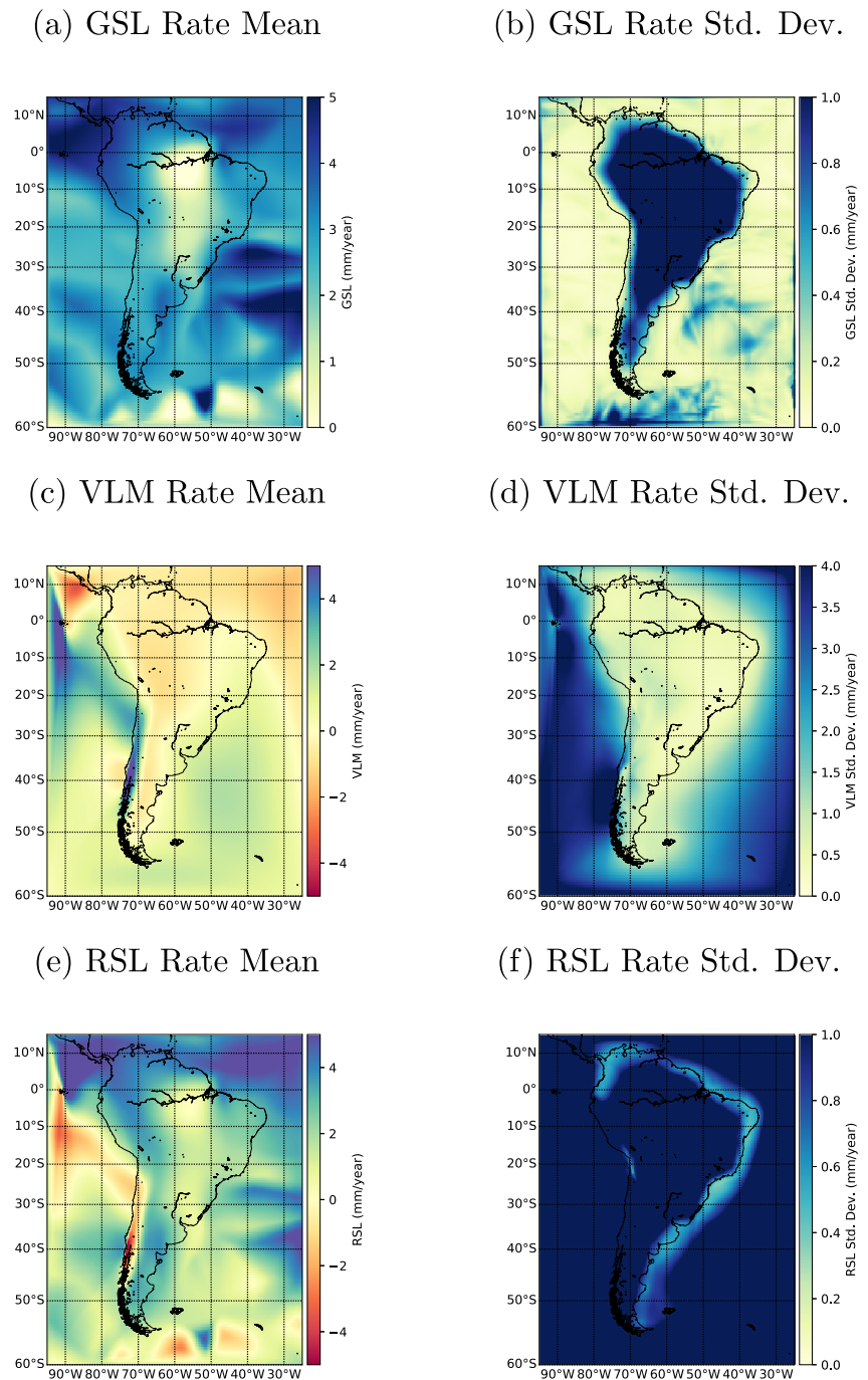
Figure 4. Ensemble mean plots for (a) GSL, (c) VLM, (e) RSL and standard deviation plots for (b) GSL, (d) VLM (f) RSL for the joint inversion of all data types for the South American region.
