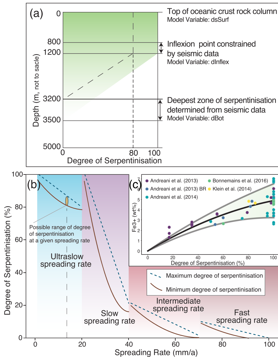
Figure 2. (a) Relationship between depth and degree of serpentinization (for ultraslow and slow ridges only), ds_{surf} , d_{inflex} , and d_{bot} refer to degree of serpentinization at surface, depth to the inflection point (when serpentinization starts to decrease linearly with depth), and depth to bottom of serpentinization, respectively. Depth values are taken from Cannat et al. (2010) and are based on seismic profiles revealing the depth and degree of serpentinization. The shaded blue area is summed and becomes our degree of serpentinization for each ridge segment. (b) Spreading rate and degree of serpentinization that are used to determine ds_{surf} in our calculations for ultraslow and slow ridges or the average degree of serpentinization at intermediate and fast ridges (since mantle peridotites are not exhumed at these ridge types); for each ridge classification (ultraslow, slow, etc.) we create an inverse relationship (blue dotted lines) between spreading rate and degree of serpentinization to act as an upper limit on the maximum possible degree of serpentinization, either at the top of the lithospheric column (in the case of slow and ultraslow ridges) or as an average throughout the column (for intermediate and fast). We introduce some variance into the model by constructing a second curve that describes the minimum degree of serpentinization (red solid lines) such that our methodology samples the resulting parameter space. We ensure that the minimum degree of serpentinization is also within the prescribed ds_{surf} bounds established from the literature. The minimum degree of serpentinization tapers at the limit of each spreading system classification (e.g., 100% and 80% for ultraslow and 80 and 20% for slow), in order to address some uncertainty in spreading rate histories of the ocean plates (i.e., a plate spreading at 19 mm/a with 10–15% uncertainty [e.g., Müller et al., 2008] might actually have been spreading at 21 mm/a, by tapering the ends we try to ensure that adjacent spreading rates result in nearly adjacent ds_{surf} values). A truncated uniform distribution of the values between the two lines (e.g., orange ellipse in (b)) is calculated per spreading rate of each ridge segment, at each time step, and a degree of serpentinization is selected at random from this range. (c) Distribution of the degree of serpentinization and wt % of ferric iron, see Supp. Material 1 for the table. Black line is mean, with gray lines one standard deviation. Data were taken from Andreani et al. (2013); Andreani et al. (2014); Bonnemains et al. (2016); and Klein et al. (2014).
