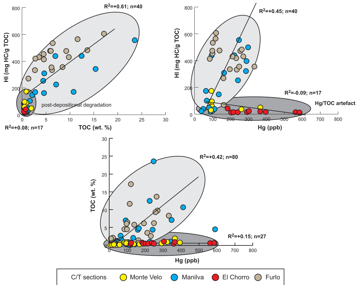
Figure 10. (a) TOC (wt.%) versus HI (mg HC/g TOC), (b) HI (mg HC/g TOC) versus Hg (ppb), and (c) TOC (wt.%) versus Hg (ppb) diagrams for the samples from Furlo, Manilva, Monte Velo, and El Chorro.
