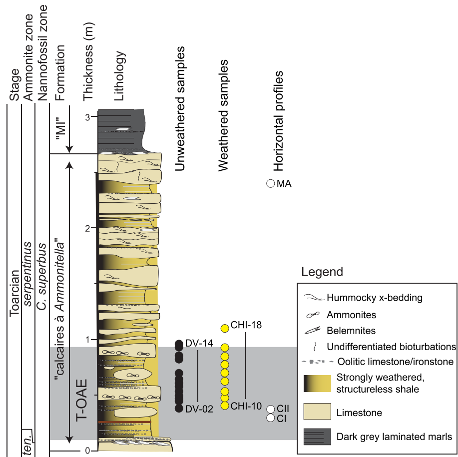
Figure 2. Lithological succession of the Lafarge cement quarry (modified after Suan et al., 2003). The biostratigraphic zonation is based on ammonites and calcareous nannofossils (Suan et al., 2013). Stratigraphic position of the weathered and unweathered bulk rock samples and horizontal profiles are shown.
