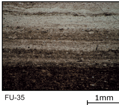
Figure 4. Microfacies photomicrographs of El Chorro, Monte Velo, Manilva, and Furlo sections showing typical laminated organic-rich layers with radiolarians, diatoms, and biogenic phosphate fragments.
