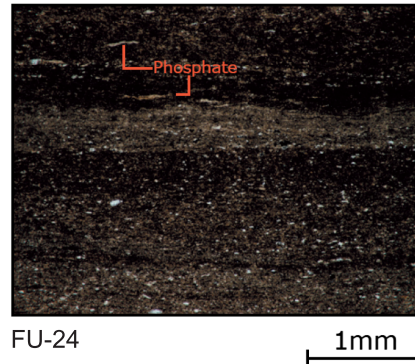
Figure 4. Microfacies photomicrographs of El Chorro, Monte Velo, Manilva, and Furlo sections showing typical laminated organic-rich layers with radiolarians, diatoms, and biogenic phosphate fragments.
