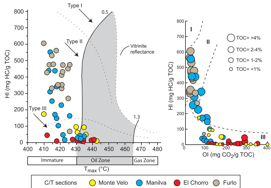
Figure 9. HI/ T_{max} diagram for preserved organic matter (OM) and cross plot between Oxygen Index (OI, mg CO 2 /g TOC) and Hydrogen Index (HI, mg HC/g TOC) for Furlo, Manilva, Monte Velo, and El Chorro sections in a modified van Krevelen-type diagram, showing the different types of organic matter (Espitalié et al., 1985).
