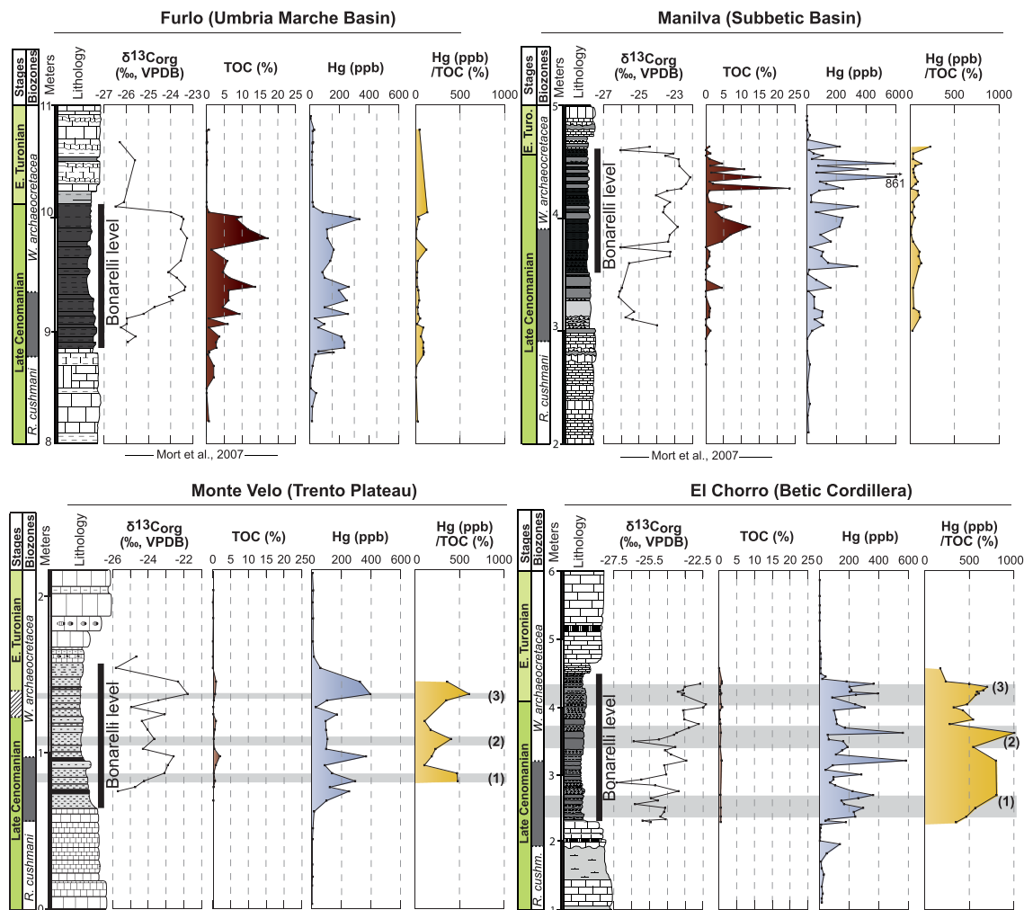
Figure 8. \delta^{13}\text{C}_{\text{org}} (‰ VPDB), total organic carbon (TOC, wt. %), Hg (ppb), and Hg/TOC (ppb/wt. %) ratios data from Furlo (Central Italy, Umbria Marche Basin), Manilva (southern Spain, Subbetic Basin), El Chorro (southern Spain, Betic Cordillera), and Monte Velo (northern Italy, Trento Plateau) sections. The precise biostratigraphic framework is based on planktonic foraminiferal assemblages (Mort et al., 2007a, 2007b).
