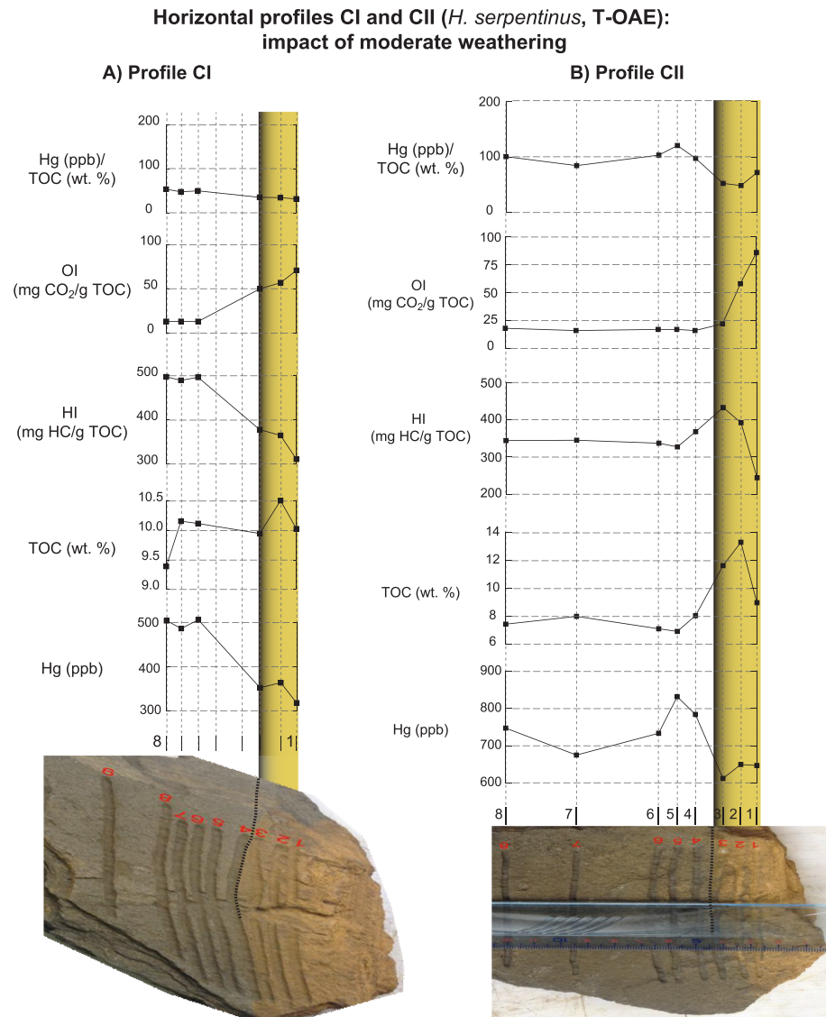
Figure 5. Hg (ppb), TOC (wt.%), HI (mg HC/g TOC), OI (mg CO 2 /g TOC), and Hg/TOC (ppb/wt.%) ratios along horizontal profiles (a) CI and (b) CII ( H. serpentinus ammonite Zone, T-OAE). The yellow bars represent the weathered edges of the horizontal horizons.
