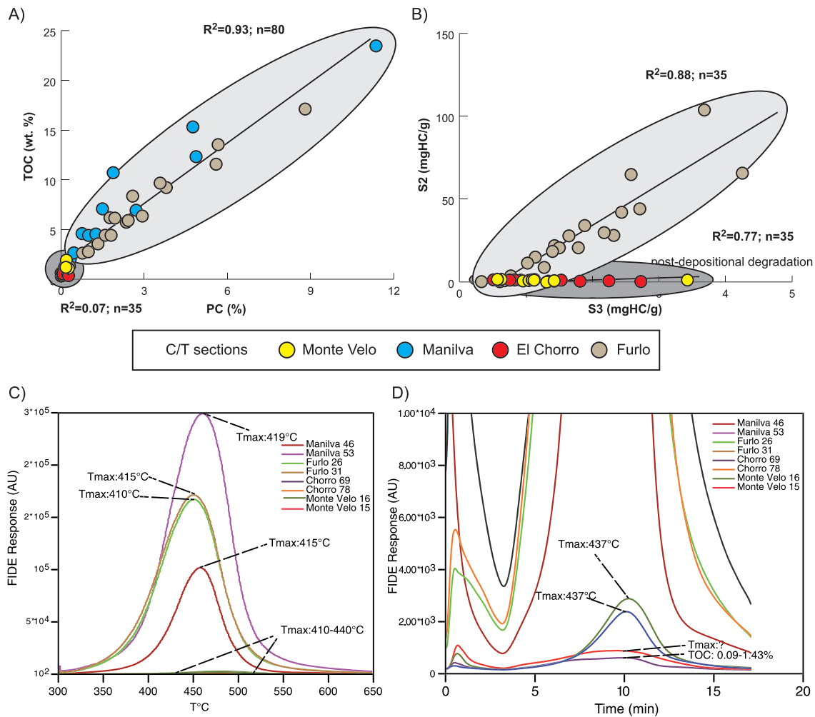
Figure 11. (a) TOC (wt.%) versus PC (%) diagram, (b) S2 (mg HC/g) versus S3 (mg HC/g) diagram, and (c) and (d) S2 thermogram for the samples from Furlo, Manilva, Monte Velo, and El Chorro.
