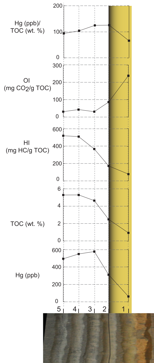
Figure 6. Hg (ppb), TOC (wt.%), HI (mg HC/g TOC), OI (mg CO 2 /g TOC), and Hg/TOC (ppb/wt.%) ratios along horizontal profile MA ( H. bifrons ammonite Zone). The yellow bars represent the weathered edges of the horizontal horizons.
