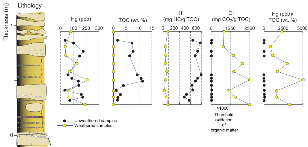
Figure 7. Hg (ppb), Total organic carbon (TOC, wt.%), HI (mg HC/g TOC), OI (mg CO 2 /g TOC), and Hg/TOC (ppb/wt.%) ratios data from (a) weathered samples, (b) unweathered samples of the T-OAE interval equivalent.
