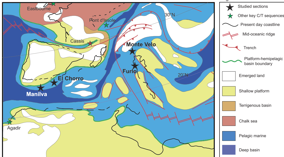
Figure 1. Palaeogeographic map of the western Tethys during the (a) Lower Toarcian (modified from Mattioli et al., 2008) and the (b) uppermost Cenomanian-lowermost Turonian (modified from Dercourt et al., 1993), showing the location of the studied sections (Lafarge cement quarry, Monte Velo, Furlo, Manilva, El Chorro).
