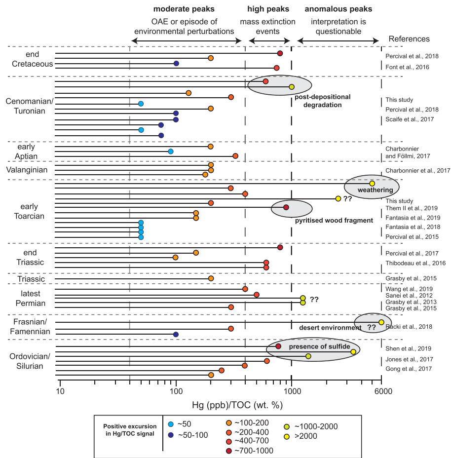
Figure 12. Reported Hg/TOC ratios across various events during the Phanerozoic time interval. The vertical dash lines represent the thresholds between anomalous (>1,000 ppb/wt.%), high (400–1,000 ppb/wt.%), and moderate (<400 ppb/wt.%) Hg/TOC ratio peaks.
