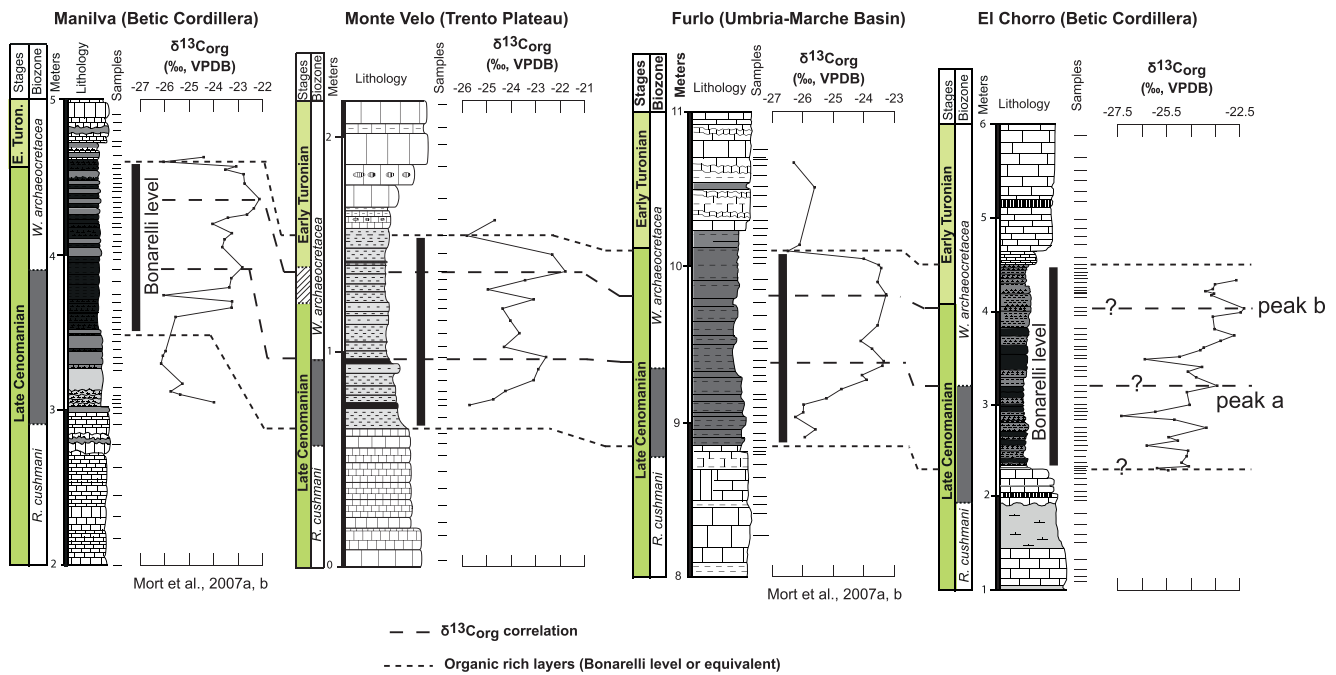
Figure 3. Stratigraphic (short-dashed line) and carbon-isotopic (dashed line) correlations of the Cenomanian/Turonian boundary interval of the Manilva (Subbetic Basin), Monte Velo (Trento Plateau), Furlo (Umbria Marche Basin), and El Chorro (Betic Cordillera) sections (Mort, Jacquat, et al., 2007a, Mort, Adatte, et al., 2007b). The biostratigraphic framework is based on planktonic foraminiferal assemblages (Mort, Jacquat, et al., 2007a, Mort, Adatte, et al., 2007b).
