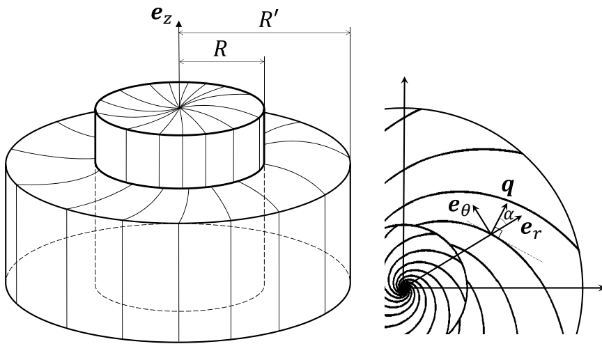
FIGURE 1. Left: The inner-cylinder of radius R rotates as a solid-body within an outer cylinder at rest. The radius R' of the outer cylinder is taken as infinite. Right: The curved lines are perpendicular to \mathbf{q} and describe logarithmic spirals. They correspond to the directions along which \sigma = \sigma^\perp and \mu = \mu^\perp .
