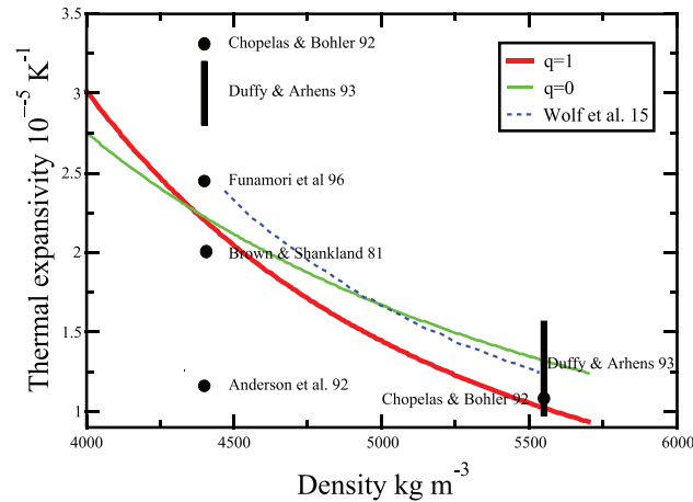
Figure 3. Thermal expansivity \alpha_a as a function of density in the Earth mantle using the parameters of Fig. 1. The predictions are with q = 1 (solid red) and q = 0 (green). Various experimental observations with conditions appropriate for the top of the lower mantle or for the CMB are indicated by dots or vertical ranges.
