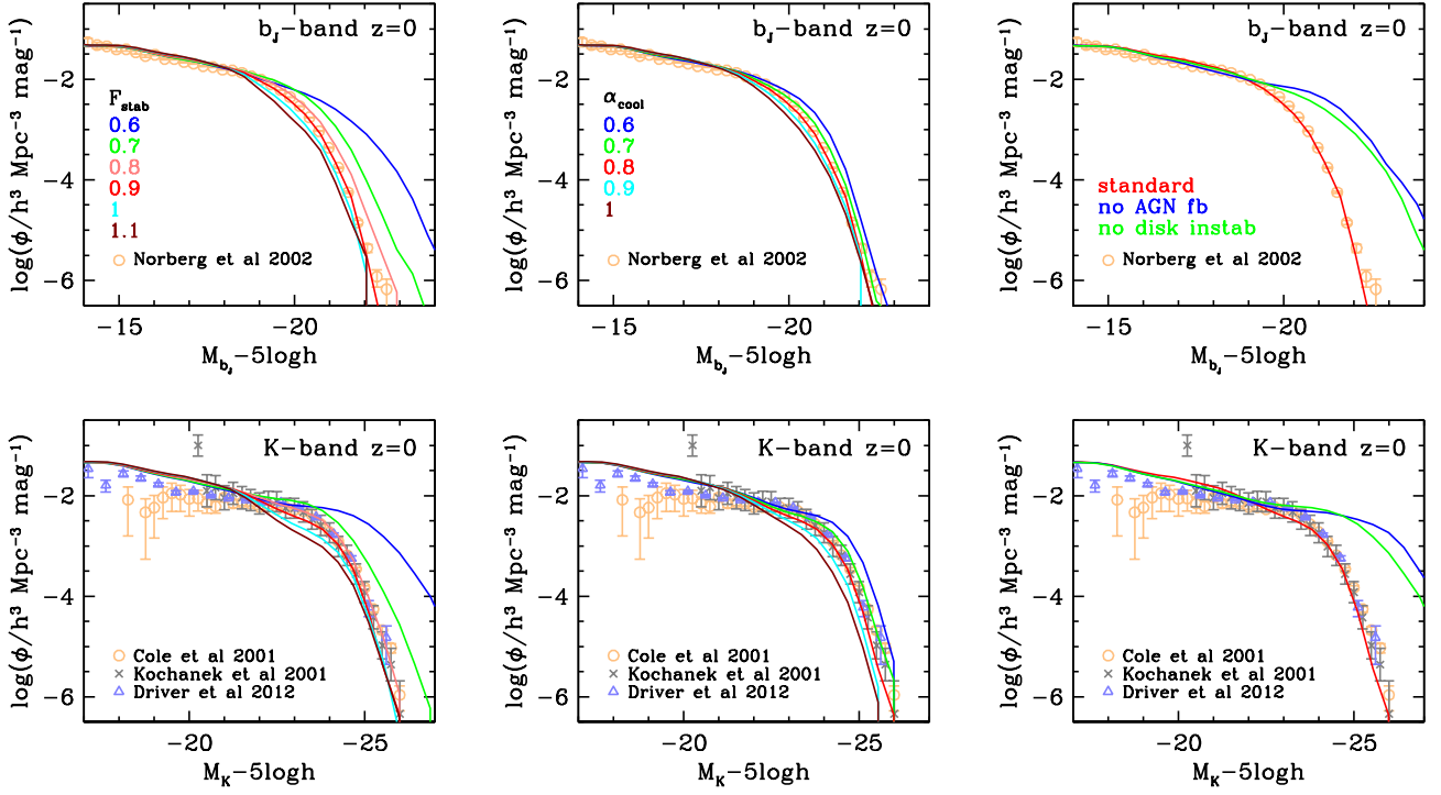
Figure C2. Effects on the b_J - and K-band LFs at z=0 of varying (a) the disc stability parameter F_{\text{stab}} , (b) the AGN feedback parameters \alpha_{\text{cool}} , and (c) of turning off AGN feedback or disc instabilities, as shown by the key in each panel. A single parameter is varied in each column, with the red curves showing the standard model.
