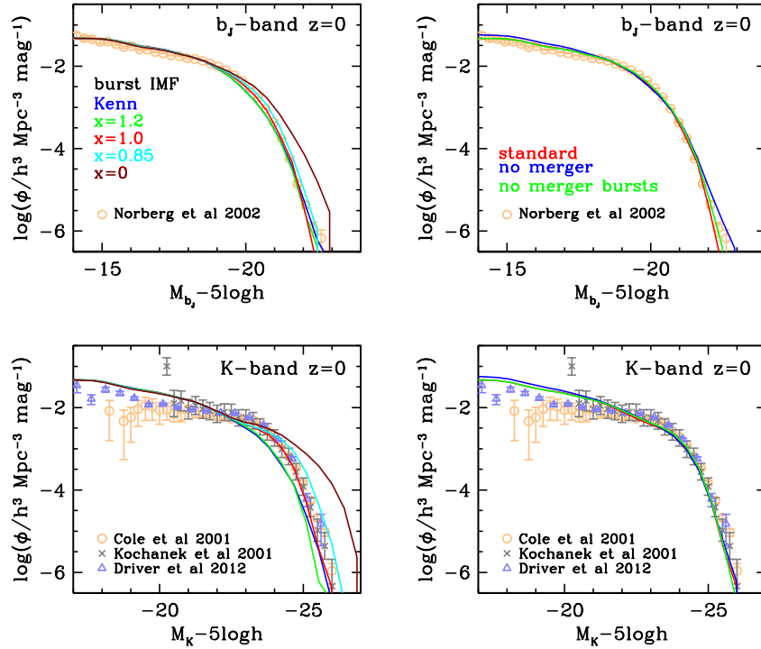
Figure C3. Effects on the b_J - and K-band LFs at z=0 of (a) changing IMF in starbursts, and (b) turning off galaxy mergers or starbursts triggered by galaxy mergers, as shown by the key in each panel. A single parameter is varied in each column, with the red curves showing the standard model.
