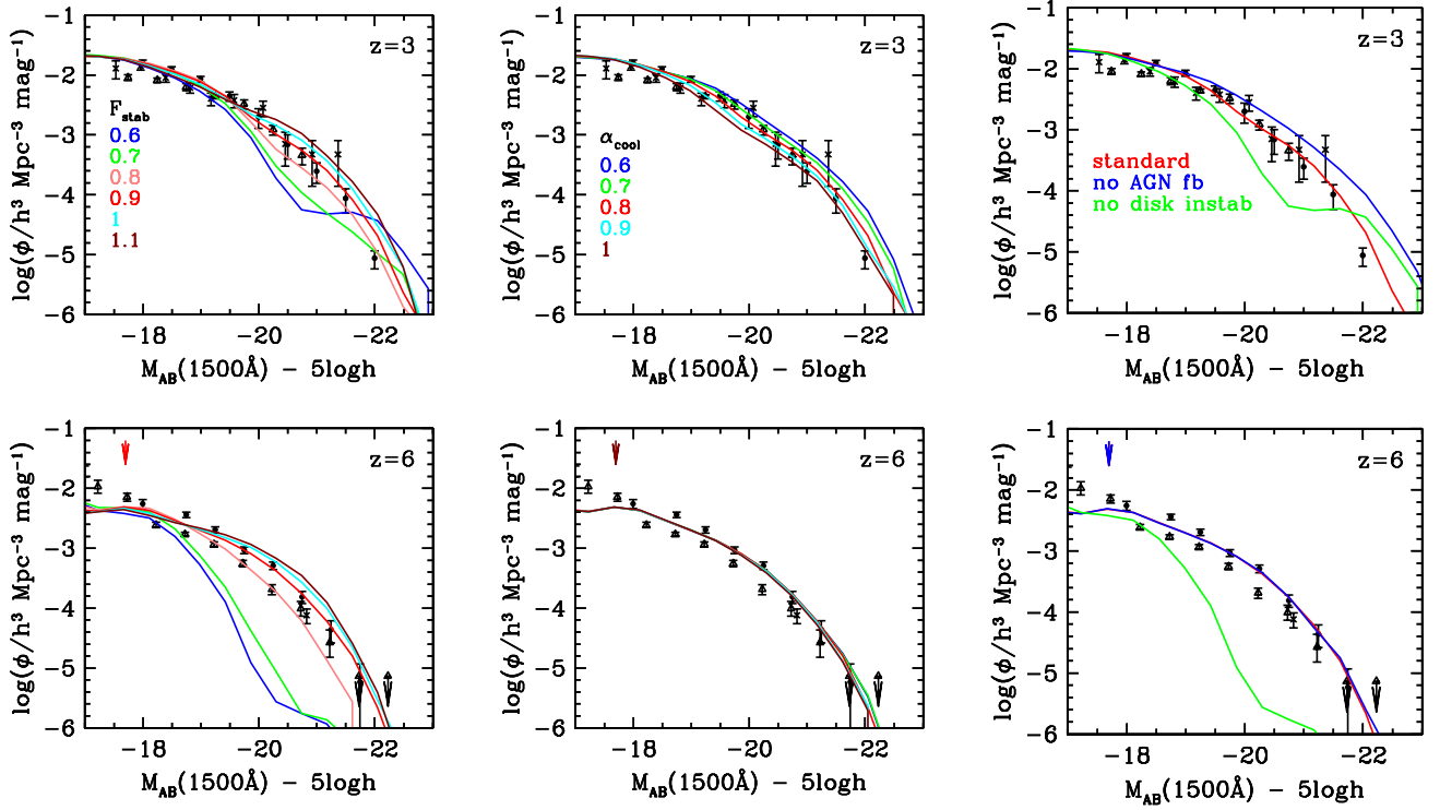
Figure C23. Effects on the rest-frame far-UV (1500 Å) LF at z = 3 and 6 of varying (a) the disc stability parameter F_{\text{stab}} , (b) the AGN feedback parameter \alpha_{\text{cool}} , and (c) of turning off AGN feedback or disc instabilities. A single parameter is varied in each column, with the red curves showing the standard model.
