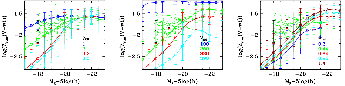
Figure C12. Effects on the stellar metallicity in early-type galaxies at z = 0 of varying the supernova feedback parameters \gamma_{\text{SN}} and V_{\text{SN}} and the gas return time-scale parameter \alpha_{\text{ret}} . The red curves show the standard model. The observational data plotted are the same as in Fig. 13.
