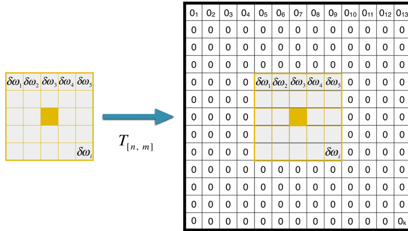
Figure A2. The matrix T_{[n,m]} for making \delta w_{[n,m]} the same length as w_{[n,m]} . The indices of \delta w_i and O_k are for the pixels (rather than the PSF correction iterations). T_{[n,m]} is a matrix at the n^{\text{th}} outer loop and the m^{\text{th}} inner loop.
