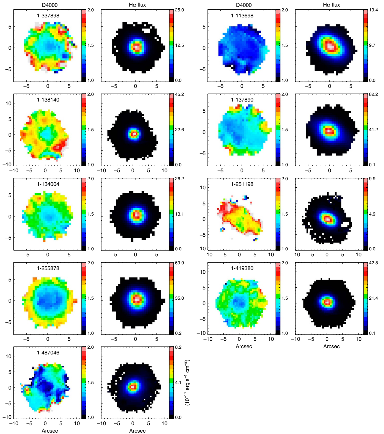
Figure 3 | The D4000 and H \alpha flux maps for nine star-forming counter rotators. The MaNGA-ID for each galaxy is shown in the D4000 map. The H \alpha flux is in the unit of 10^{-17} \text{ erg s}^{-1} \text{ cm}^{-2} .
