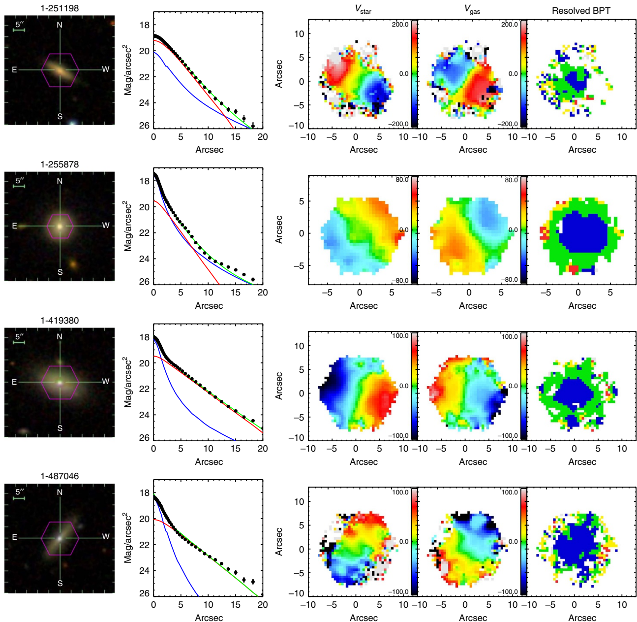
Figure 7 | Properties of the blue counter rotators. Same as Fig. 6, but with more objects.
