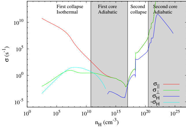
Fig. 4. Conductivities as a function of density for the fiducial case. Light blue: negative Hall conductivity, dark blue: positive Hall conductivity, red: parallel conductivity, green: perpendicular conductivity.
