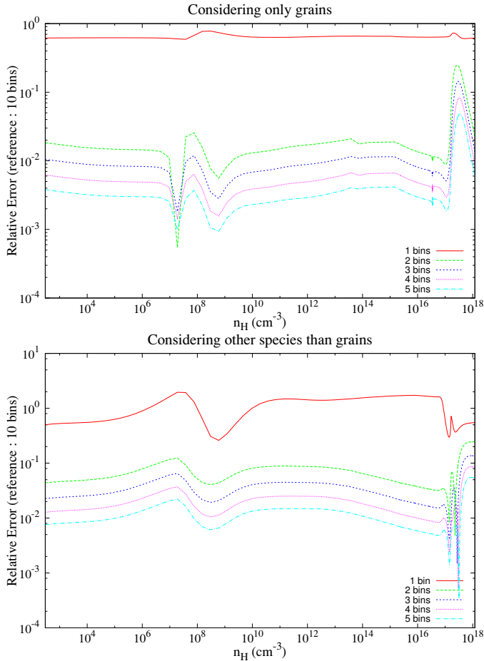
Fig. 10. Relative error in the species abundances ( = \frac{\|x_{N_{\text{bins}}} - x_{\text{ref}}\|}{\|x_{\text{ref}}\|} ) for different numbers of size bins (relatively to the ten bins results) for grains only ( top panel ), and for other species ( bottom panel ) in the density range before grain evaporation.
