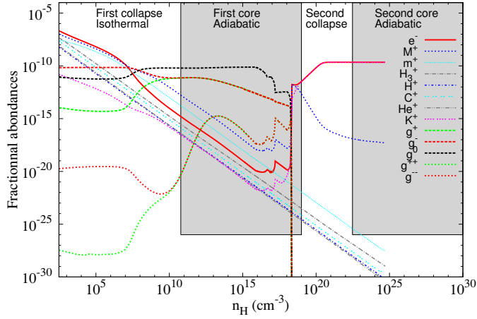
Fig. B.1. Abundances of the chemical species with double-charge grains, without Na, the thermal ionisation of H and the thermionic emission.
