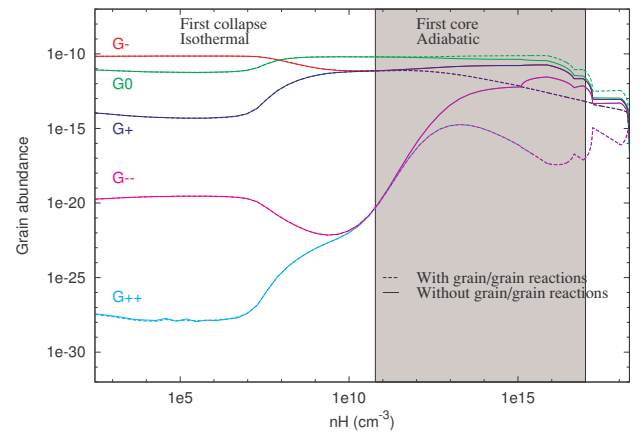
Fig. B.4. Comparison of the grain abundances with (dashed lines) and without (solid lines) charge transfer between grains for singly charged grains (top panel) and singly and doubly charged grains (bottom panel).
