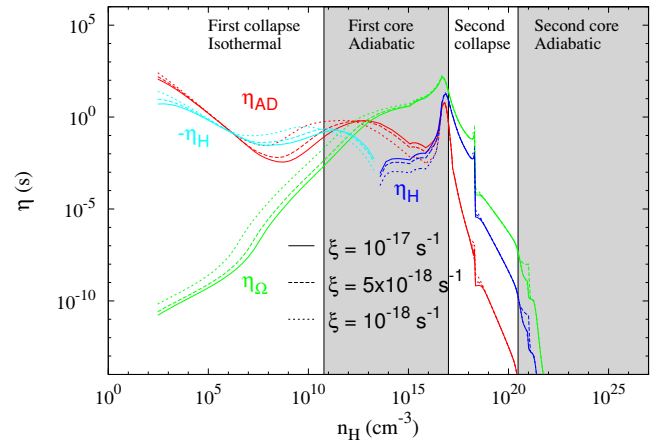
Fig. 9. Resistivities for different cosmic-ray ionisation rates, with the barotropic EOS. Solid lines: fiducial value \zeta_{\text{CR,ref}} = 1 \times 10^{-17} \text{ s}^{-1} . Dashed lines: \zeta_{\text{CR}} = \frac{\zeta_{\text{CR,ref}}}{2} = 5 \times 10^{-18} \text{ s}^{-1} . Dotted lines: \zeta_{\text{CR}} = \frac{\zeta_{\text{CR,ref}}}{10} = 1 \times 10^{-18} \text{ s}^{-1} . Same colour coding as Fig. 5.
