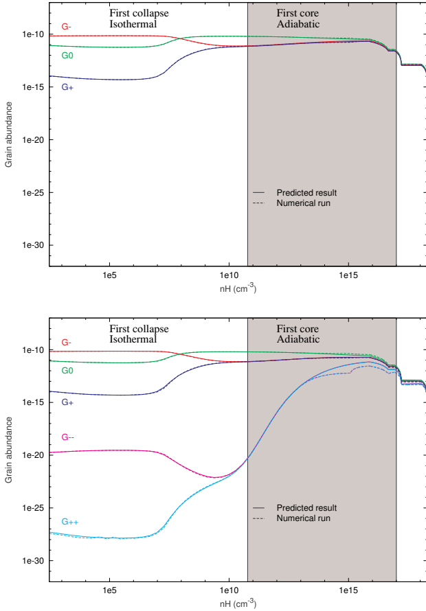
Fig. B.5. Comparison of the abundances of grains computed with our code (dashed lines) and predicted from the ions and electron abundances (solid lines) for singly charged grains ( top panel ) and singly and doubly charged grains with one bin ( bottom panel ).
