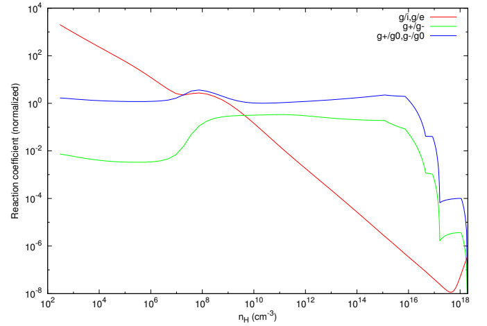
Fig. B.3. Highest reactions rates for grain/ion and grain/electron reactions (red curve), positively charged grain/negatively charged grain reactions (green curve) and neutral grain/charged grain reactions (blue curve).
