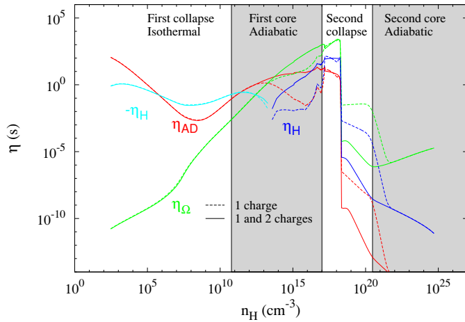
Fig. B.2. Resistivity comparison for the simplified case. Dashed line: network with only singly charged grains, solid line: network with singly and doubly charged grains.
