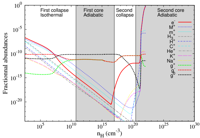
Fig. 7. Fractional abundances, using ten bins, without grain evaporation.
