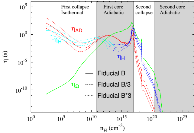
Fig. 6. Resistivities as a function of density for the fiducial case, and a magnetic field three times higher and lower. Same colour coding as Fig. 5.
