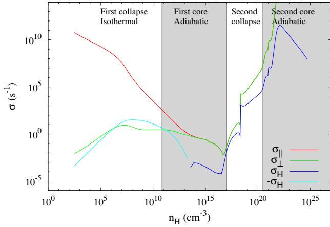
Fig. 4. Conductivities as a function of density for the fiducial case. Light blue: negative Hall conductivity, dark blue: positive Hall conductivity, red: parallel conductivity, green: perpendicular conductivity.
