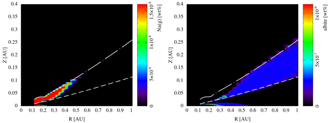
Figure 6. Resulting chemical distribution from our 2D model for Na(g), left, and albite (NaAlSi 3 O 8 ), right. The dashed line is the \tau = 1 surface of the disc and the dash–dotted line represents the disc surface.
