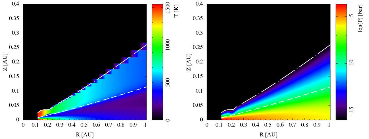
Figure 1. Resulting disc structure from the D’Alessio et al. (1998) model. Left: temperature distribution. Right: pressure distribution. The dashed line is the \tau = 1 surface of the disc and the dash–dotted line represents the disc surface.
