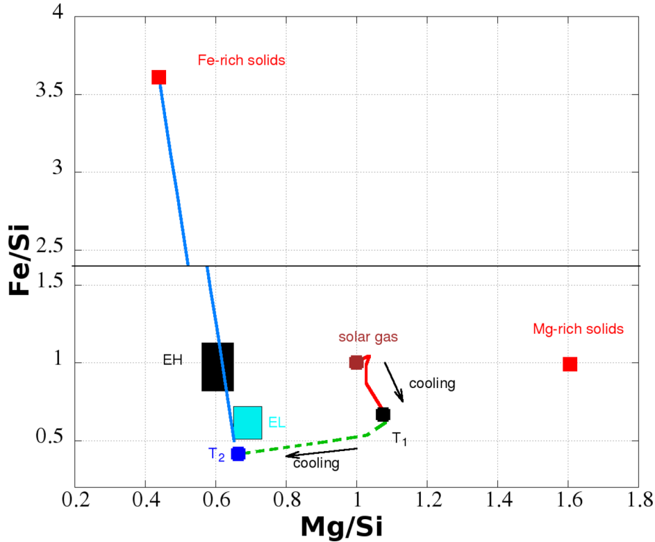
Figure 5. Resulting Mg/Si versus Fe/Si ratios normalized to solar values from our toy model for: the initial solar gas mix, the EHs and ELs from Sears (1997), the T_1 and T_2 fractionated gas from Table 1, the Fe-rich solids removed after the first condensation from T_0 to T_1 , and the Mg-rich solids removed after the second condensation from T_1 to T_2 . The mixing line between the T_2 gas and the Fe-rich solids is also drawn. The red continuous line shows how the gas with solar composition would fractionate across the temperature range from T_0 (solar) and T_1 , while the green dashed line shows how the T_1 gas would fractionate from T_1 to T_2 .
