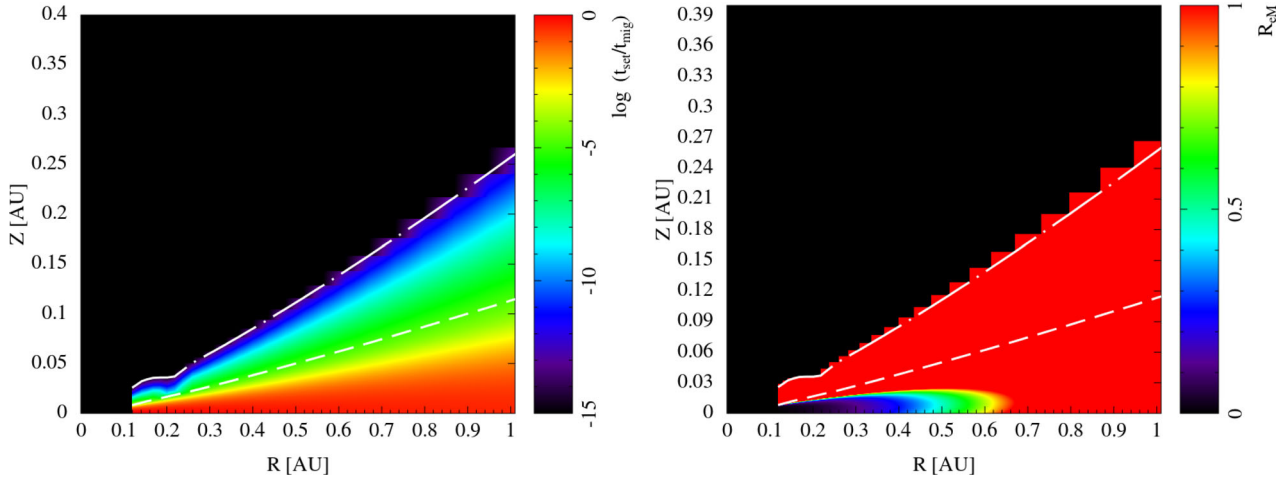
Figure 3. Dynamical distribution maps: left, \log BI_{part}BI_{hypset}/\tau_{mig} , and right, R_{EM} for 0.1 \mu\text{m} -sized grain. The dashed line is the \tau = 1 surface of the disc and the dash-dotted line represents the disc surface.
