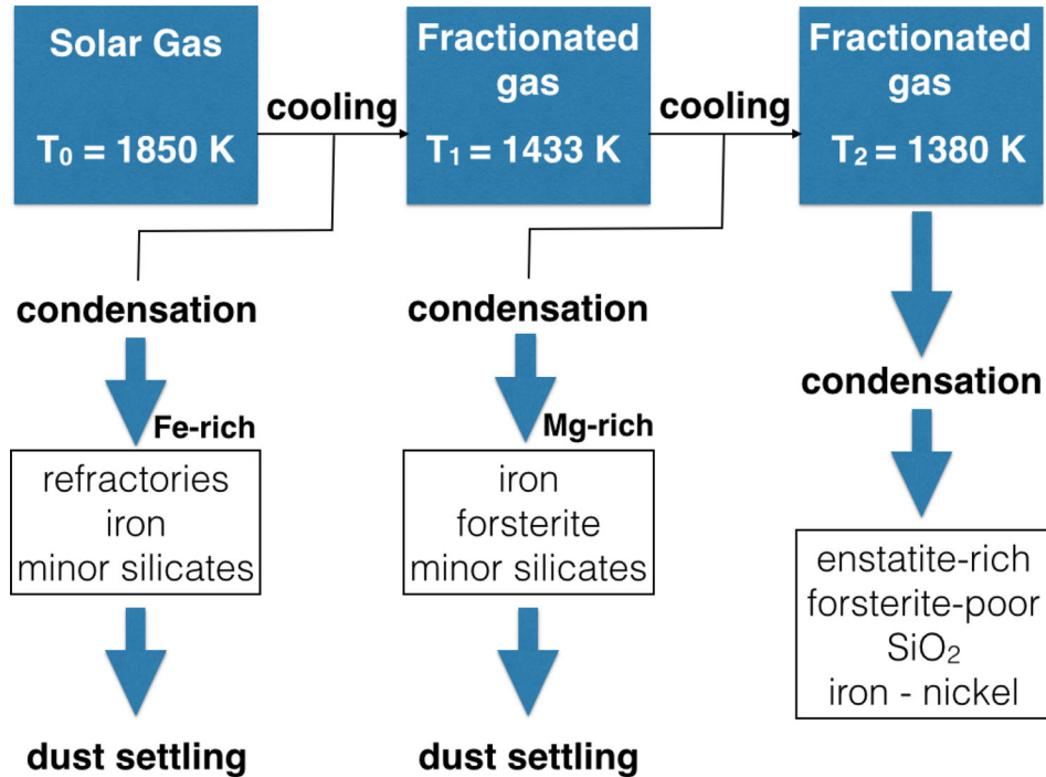
Figure 4. Schematic summarizing the gas fractionation due to the vertical settling of dust. A parcel of gas with solar composition (at constant pressure of P = 10^{-3} bar and initial temperature of T_0 = 1850\text{ K} ) is cooled to T_1 = 1433\text{ K} and all the solids which condense at this temperature are removed from the environment due to the efficient vertical dust settling. The fractionated T_1 gas is then further cooled to T_2 = 1380\text{ K} , where it reaches the condensation temperature of forsterite. Forsterite, iron and minor silicates are efficiently removed from the environment, and the resulting fractionated gas has Mg/Si and Fe/Si ratios of 0.66 and 0.41, respectively. Further condensation of the T_2 gas leads to enstatite-rich condensates.
