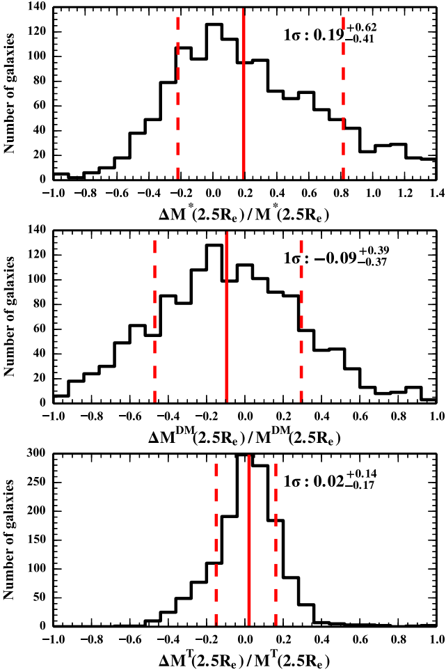
Figure 7. Histogram of the mass error for the 1413 simulated galaxies with low-resolution images. Upper: enclosed stellar mass error \Delta M^*(2.5 R_e)/M^*(2.5 R_e) . Middle: enclosed dark matter error \Delta M^{\text{DM}}(2.5 R_e)/M^{\text{DM}}(2.5 R_e) . Lower: enclosed total mass error \Delta M^{\text{T}}(2.5 R_e)/M^{\text{T}}(2.5 R_e) . The labels and legends are the same as in Fig. 5.
