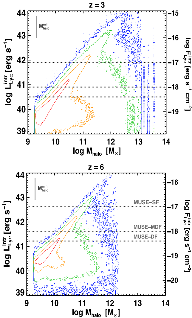
Figure 3. Intrinsic Ly \alpha luminosity versus halo mass at z = 3 (top panel) and z = 6 (bottom panel). Contours show the number distribution of galaxies in the model. The vertical line in the top-left corner illustrates the halo mass resolution limit of the simulation ( M_{\text{halo}}^{\text{min}} = 2 \times 10^9 M_{\odot} ). The dotted lines correspond to the Ly \alpha flux limits of typical MUSE SF, MDF and DF surveys. The brightest Ly \alpha -emitting galaxies residing in the least massive DM haloes in our model have an approximate intrinsic Ly \alpha luminosity of 2 \times 10^{40} erg s ^{-1} and 7 \times 10^{40} erg s ^{-1} at z = 3 and 6 , respectively (namely, a Ly \alpha flux of \approx 2 \times 10^{-19} erg s ^{-1} cm ^{-2} at both redshifts). We consider that the sample of Ly \alpha -emitting galaxies is complete above these values.
