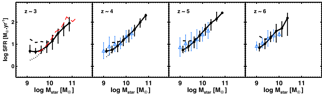
Figure 2. Relation between stellar mass ( M_{\text{star}} ) and SFR at z \approx 3, 4, 5, and 6 . In black, we show the median SFR per bin of stellar mass along with the 10th–90th percentiles for galaxies with 10^9 < (M_{\text{star}}/M_{\odot}) < 10^{11} . The dotted, solid, and dashed curves correspond to UV magnitude cuts of M_{1500} < -19 , M_{1500} < -20 , and M_{1500} < -21 , respectively. The red dashed line and the blue triangles correspond to the data from Kajisawa et al. (2010) and Salmon et al. (2015), respectively.
