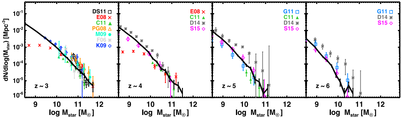
Figure 1. SMF at z \approx 3, 4, 5, and 6 . The solid black line with Poisson error bars corresponds to our model and the symbols are observational estimates (converted to our IMF) from Domínguez Sánchez et al. (2011, DS11), Elsner, Feulner & Hopp (2008, E08), Caputi et al. (2011, C11), Pérez-González et al. (2008, PG08), Marchesini et al. (2009, M09), Fontana et al. (2006, F06), Kajisawa et al. (2009, K09), González et al. (2011, G11), Duncan et al. (2014, D14), and Song et al. (2015, S15).
