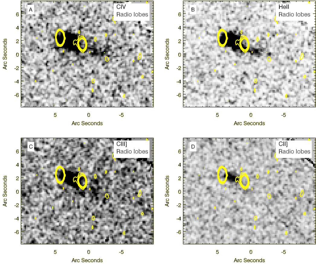
Fig. 7. Continuum subtracted moment-0 maps of the CIV, HeII, CIII], and CII] emission lines. The continuum is determined from the nearby line free channels for each line. Panel A): sum over the CIV emission line for the wavelength range \lambda_{\text{obs}} = 6050\text{--}6090 \text{ \AA} . Panel B): sum over the HeII emission line for the wavelength range \lambda_{\text{obs}} = 6422\text{--}6430 \text{ \AA} and is the same image as the blue colour of the middle panel of Fig. 5. Panel C): sum over the CIII] emission line for the wavelength range \lambda_{\text{obs}} = 7455\text{--}7485 \text{ \AA} . Panel D): sum over the CII] emission line for the wavelength range \lambda_{\text{obs}} = 9071\text{--}9171 \text{ \AA} . Over-plotted with yellow contours in all panels is the VLA radio map, as a reference.
